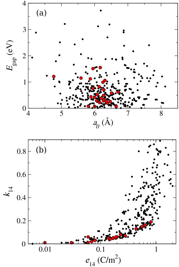
FIG. 2 (color online). (a) Cell parameters (in Å) of insulating ABC combinations as well as their range of band gaps (in eV) are depicted as black circles. (b) Electromechanical coupling factor k_{14} of insulating ABC combinations as a function of piezoelectric constant e_{14} . Known combinations, from Table I, are highlighted as (bigger) filled red circles.
