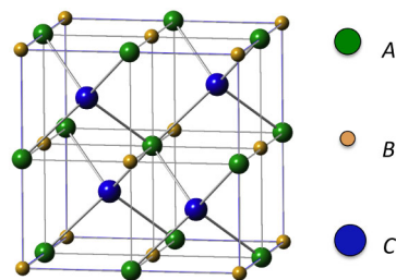
FIG. 1 (color online). The ABC half-Heusler structure: A (green, big circles) and B (orange, small circles) are arranged in a rocksalt lattice, with the tetrahedral coordination of C (blue, biggest circles) by A shown.
