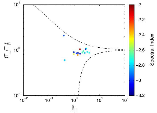
FIG. 4 (color online). Spectral index ( 3 < k\rho_i < 15 ) as a function of ion temperature anisotropy and ion parallel beta. The upper dashed line is the mirror instability threshold, and the lower dashed line is the oblique fire hose instability threshold from Ref. [78].
