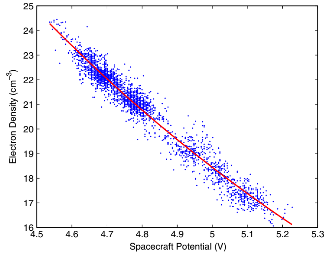
FIG. 1 (color online). Electron density, n_e , as a function of the spacecraft potential relative to the solar wind, V_{sc} . The best fit exponential calibration curve is shown as a solid red line.
