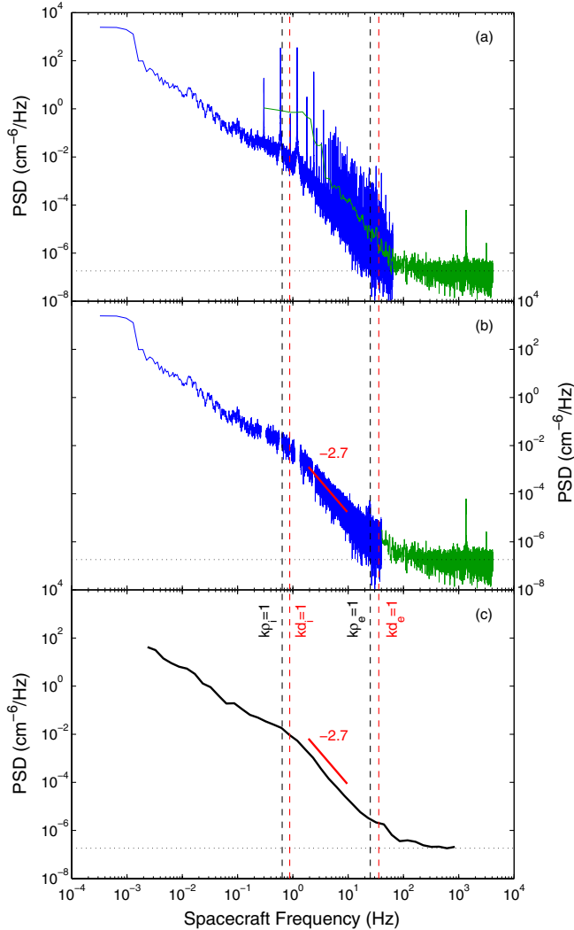
FIG. 2 (color online). Power spectra of electron density fluctuations: (a) from calibrated data (artificial spikes present), (b) with artificial spikes removed, (c) smoothed. Ion and electron gyro-scales, \rho , and inertial lengths, d , are marked with vertical dashed lines. The empirical noise floor is marked with a horizontal dotted line.
