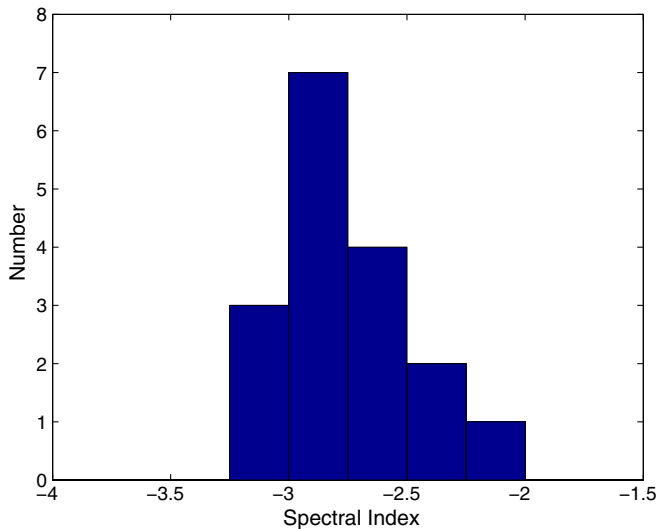
FIG. 3 (color online). Histogram of electron density spectral index values between ion and electron scales ( 3 < k\rho_i < 15 ).
