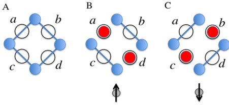
FIG. 4 (color online). Proposed design of the quantum switch in cold atomic systems. Between the end sites of the four half-chains, four quantum wells a , b , c , d are positioned. When empty, they do not affect the tunneling between the end sites (a). Two dipolar molecules (red circles) interacting via long-range repulsive interactions with each other are put in the quantum wells (b),(c). The ground state of the molecules is doubly degenerate, corresponding to the occupation of either a , c wells (b) or b , d wells (c), such that the repulsive interactions between them are minimized. The dipolar molecules are assumed to be interacting with the particles constituting the many-body chains, such that depending on their state they can block the tunneling between neighboring sites (b),(d). The two states represent the |\uparrow\rangle and |\downarrow\rangle states of the quantum switch.
