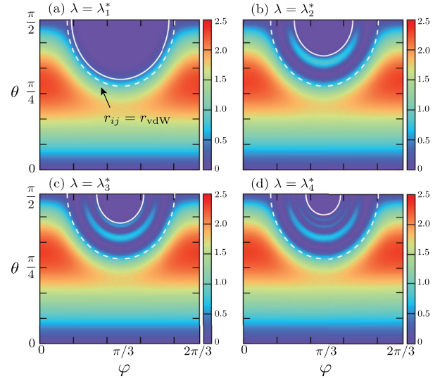
FIG. 2 (color online). Density plot of the three-body probability density |\Phi_\nu(R; \theta, \varphi)|^2 \sin 2\theta which determines the three particle configuration [see Fig. 1(c)] in the \theta - \varphi hyperangular plane for a fixed R ( \sin 2\theta is the volume element). (a)–(d) show the results for an R near the minima of the Efimov potentials in Fig. 1(b) for the first four scattering length poles of the v_\lambda^a model as indicated. (a) shows that there is a negligible probability to find the particles at distances smaller than r_{\text{vdW}} (outer dashed circle) and, of course, inside the 1/r^{12} repulsive barrier (inner solid circle). For higher poles, i.e., as the strength of the hardcore part of the v_\lambda^a potential decreases, the potential becomes deeper and penetration into the region r < r_{\text{vdW}} is now classically allowed. Nevertheless, (b)–(e) show that inside-the-well suppression still efficiently suppresses the probability to find particle pairs at distances r < r_{\text{vdW}} , found to be in the range 2%–4%.
