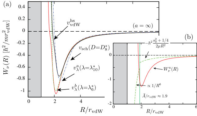
FIG. 3 (color online). (a) Efimov potential obtained from the different two-body potential models used here. The reasonably good agreement between the results obtained using models supporting many bound states ( v_{\text{sch}} , v_\lambda^a and v_\lambda^b ) and v_{\text{vdW}}^{\text{hs}} [obtained by replacing the deep potential well with a hard wall but having only one (zero-energy) bound state] supports our conclusion that the inside-the-well suppression of the wave function is the main physical mechanism behind the universality of the three-body effective potentials. The differences between these potentials are seen to cause differences of a few percent in the three-body parameter. (b) Comparison between the effective potential proposed by Ref. [39] (green dashed curve) and the one (red solid curve) constructed to describe our findings: 2\mu r_{\text{vdW}}^2 W_v^u(R)/\hbar^2 \approx -(s_0^2 + 1/4)/X^2 - b_3/X^3 - b_4/X^4 - b_5/X^5 + b_{16}/X^{16} , where X = R/r_{\text{vdW}} and b_3 = 2.334 , b_4 = 1.348 , b_5 = 44.52 , b_{16} = 4.0 \times 10^4 .
