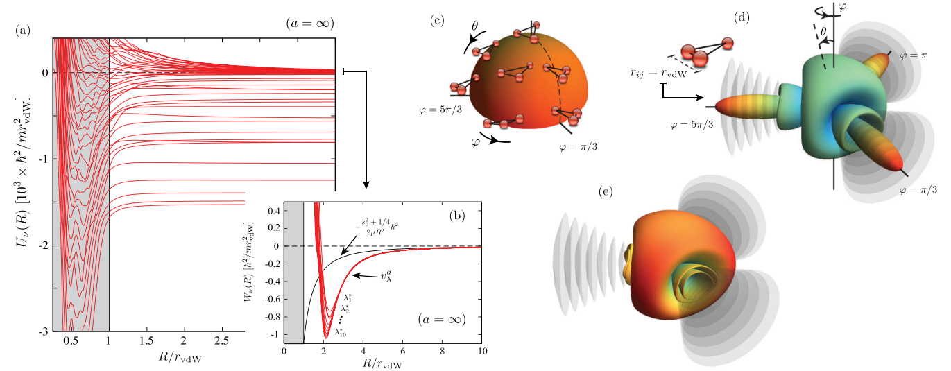
FIG. 1 (color online). (a) Full energy landscape for the three-body potentials at a = \infty for our v_\lambda^a model potential. (b) Effective diabatic potentials W_\nu relevant for Efimov physics for v_\lambda^a with an increasingly large number of bound states ( \lambda_n^* is the value of \lambda that produces a = \infty and n s -wave bound states). The W_\nu converge to a universal potential displaying the repulsive barrier at R \approx 2r_{\text{vdW}} that prevents particles’ access to short distances. (c)–(e) demonstrate the suppression of the wave function inside the potential well through the channel functions \Phi_\nu(R; \theta, \varphi) for R fixed near the minima of the Efimov potentials in (b). (c) shows the mapping of the geometrical configurations onto the hyperangles \theta and \varphi . (d) and (e) show the channel functions, where the “distance” from the origin determines |\Phi_\nu|^{1/2} , for two distinct cases: in (d) when there is a substantial probability to find two particles inside the potential well (defined by the region containing the gray disks) and in (e) with a reduced probability—see also our discussion in Fig. 2. In (d) and (e), we used the potentials v_{\text{sch}} and v_\lambda^a , respectively, both with n = 3 .
