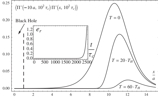
FIG. 2. Plot of the momentum-momentum correlation for x_1 = -10a and t = 100\tau_c . The profile parameters are v_{\min} = 0.9 , v_{\max} = 1.1 . It is shown for different temperatures. Inset: Relative contribution of the correlation due to the environment as a function of time, in units of the collapse time \tau_c .
