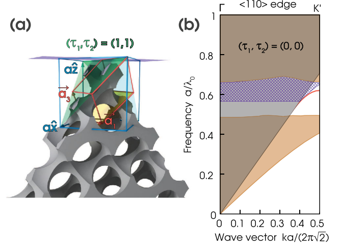
FIG. 2 (color online). (a) One unit cell of the edge waveguide along \vec{a}_1 . The 3D PhC consists of air spheres of diamond lattice in a dielectric matrix rendered in gray solid. The cells and \{111\} surfaces are the same as those in Fig. 1(a). The top purple area in the cubic cell (001) plane is the region where the 2D cuts are made in Fig. 4 and in the Supplemental Material [22]. (b) Band structure of the edge waveguide formed by two \langle 110 \rangle surfaces, both of zero termination parameters.
