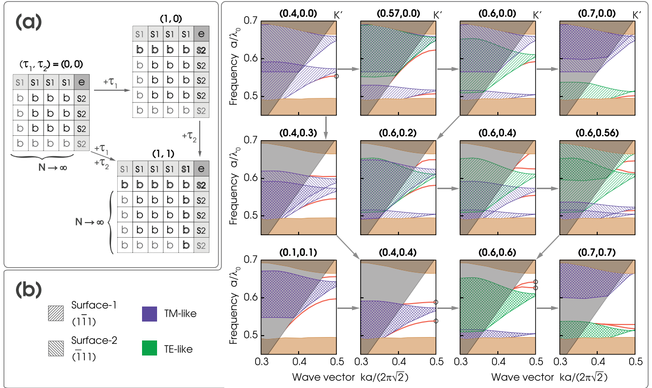
FIG. 3 (color online). (a) Schematic illustration of the periodic evolution of the edge unit cell. The cells of the outlined font indicate the increment from the original structure. By dashed the left and bottom boundaries of the structures, we mean the spatial extension of the cells beyond what is drawn. (b) Evolution of the edge dispersion diagrams of different surface terminations. The mode profiles of the circled edge dispersions at the zone boundary ( K' ) are presented in Fig. 4 and in the Supplemental Material [22].
