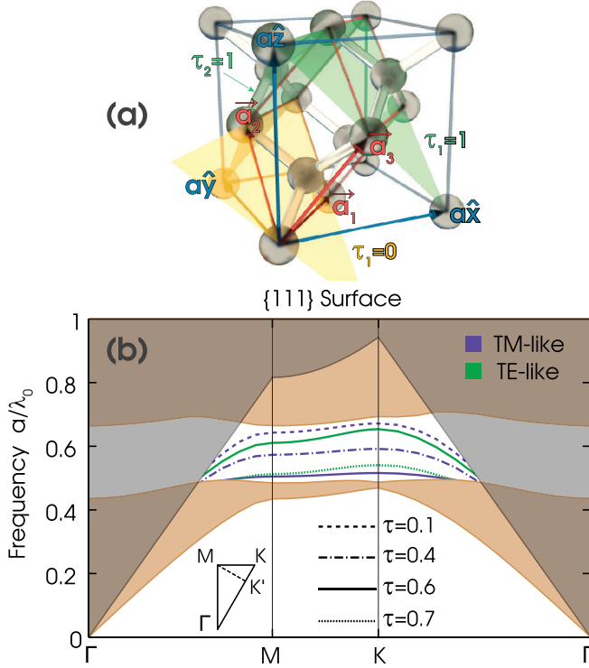
FIG. 1 (color online). (a) Illustration of a diamond lattice. The cubic unit cell of length a is outlined in blue and the fcc primitive cell is outlined in red. Two (\bar{1}\bar{1}1) surfaces of equivalent termination parameters \tau_1 = 0 and \tau_1 = 1 are shown in yellow and green. They lie on the end faces of the fcc primitive cell connected by \vec{a}_3 . The (\bar{1}\bar{1}1) surface of \tau_2 = 1 is also shown in green. Any of the two intersecting planes define the [110] edge along \vec{a}_1 . \hat{v} ( =\frac{\vec{v}}{|\vec{v}|} ) represents a unit vector along \vec{v} . (b) The projected band structure of the \{111\} surfaces of the inverse diamond PhC in air. The \{111\} surfaces, containing a C_{3v} symmetry, have a triangular lattice of lattice constant a/\sqrt{2} . The brown area is the projected bulk modes. The light cone is shaded in transparent gray. The irreducible BZ is shown as an inset. \Gamma -K' is the irreducible BZ of the edge waveguide along the \langle 110 \rangle directions.
