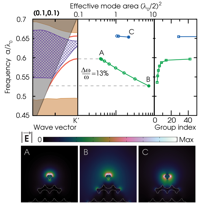
FIG. 5 (color online). Effective mode areas and group indices of the edge modes of the (0.1, 0.1) edge are evaluated over their operational bandwidths. Field profiles are plotted for three representative modes with the gray outlines of the dielectric-air interfaces.
