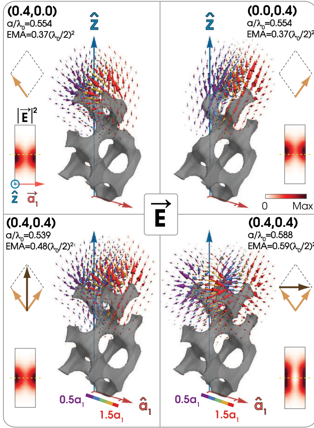
FIG. 4 (color online). Mode profiles of the edge modes associated with the TM-like surface bands at the BZ boundary ( K' ). The dielectric-air interfaces are drawn as transparent contour surfaces in gray. The arrows point to the directions of the electric fields; their sizes represent the field amplitudes. The colors of the arrows represent the field locations along the waveguide propagation direction ( \hat{a}_1 ). The fields of the amplitudes one order of magnitude less than the maximum field amplitude are not plotted. The insets on the sides of the vector plots are the plane cuts of the intensity square of the electric fields. The area and location of the plane (in air) is illustrated in Fig. 2(a). Central lines are drawn in yellow dash to indicate the mode positions.
