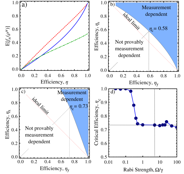
FIG. 1 (color online). (a) As a function of efficiency \eta , we plot: (red dashed) E[(\langle\hat{\sigma}_x\rangle^S)^2] for the SAID unraveling, large \Omega limit; (solid blue) E[(\langle\hat{\sigma}_y\rangle^Y)^2 + (\langle\hat{\sigma}_z\rangle^Y)^2] for the Y-homodyne unraveling, in the large \Omega limit; (green dot-dashed) E[(\langle\hat{\sigma}_x\rangle^S)^2] for the X-homodyne unraveling from simulations with \Omega = 5\gamma . (b) S^{S,Y}(\eta_Y, \eta_S) is plotted with the blue shaded regime ( S > 1 ) representing when the experiment would rule out all theories of objective atomic state reduction. (c) is the same as (b) with SAID replaced by X-homodyne detection and \Omega = 5\gamma for both unravelings. (d) The efficiency required for X and Y homodyne to have S > 1 , as a function of \Omega/\gamma . For more details see text.
