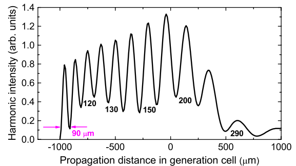
FIG. 1 (color online). On-axis variation of the H111 along the propagation direction generated by the IR pulse. The width of several Maker fringes = 2L_{\text{coh}} is indicated in \mu m, other parameters are in the text.
