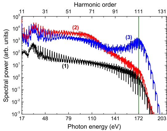
FIG. 5 (color online). Logarithmic plot of HH spectra. Black (1): harmonic spectrum generated with IR-only after 20\ \mu\text{m} propagation. Red (2): IR-only spectrum at the position of max. H111 intensity ( -40\ \mu\text{m} ). Blue (3): spectrum obtained with THz-assisted HHG at the position of max. H111 intensity ( +260\ \mu\text{m} ). THz pulse was linearly chirped such to best match the on-axis periodicity of H111 (172 eV). Vertical line: position of H111.
