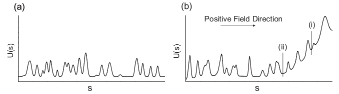
FIG. 4. Schematics of energy functions U(s) for domain wall displacements, s . (a) Position of a domain wall, with random potentials and without asymmetry. (b) Position of a domain wall after a strong electric field is applied towards the right-hand side (positive) in (i); deaged position of a domain wall in (ii).
