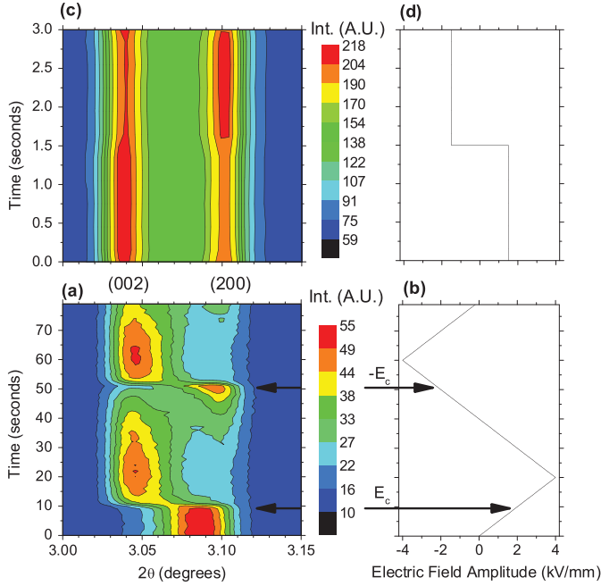
FIG. 2 (color). (a) Diffraction intensities of \{002\} reflections parallel to the electric field amplitude during (b) application of a bipolar triangular wave. (c) Diffraction intensities of \{002\} reflections parallel to the electric field amplitude during (d) application of a square bipolar electric field of 1.5 kV/mm and frequency 0.33 Hz.
