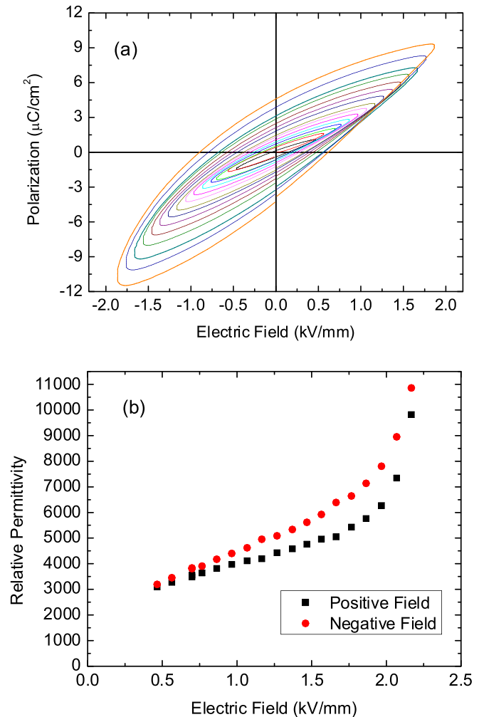
FIG. 1 (color online). (a) Polarization of BS-64PT to varying electric field amplitudes. (b) Relative permittivity measured in the positive and negative field directions as a function of electric field amplitude.
