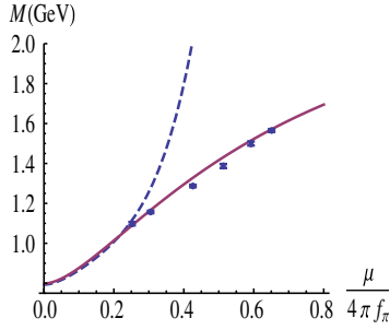
FIG. 2 (color online). Nucleon mass as a function of \mu . Square blocks: LHP lattice data [35]. Solid line: \Sigma_\pi of Eqs. (17), (9), and (13). Dashed line: Chiral approximation \tilde{\Sigma}_\pi = \tilde{\Sigma}_\pi(N) + \tilde{\Sigma}_\pi(\Delta) , Eqs. (10) and (14).
