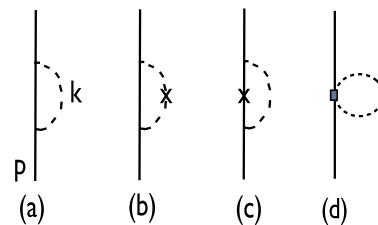
FIG. 1 (color online). (a) Pionic (dashed line) contribution to the nucleon (solid line) self-energy. (b) External interaction x with the pion. (c) External interaction x with the intermediate nucleon. (d) Effect of 2\pi -nucleon interaction.
