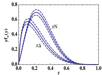
FIG. 3 (color online). y f_\pi(y) for the intermediate \pi N and \pi \Delta states for M_A = 0.99, 1.03, 1.07 GeV.
