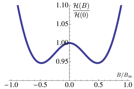
FIG. 1 (color online). The energy density (10) for \theta = 0 and \epsilon_0 E_0 = 1.3\epsilon E_{\text{crit}} , which is slightly above the critical value \epsilon_0 E_0 = \epsilon E_{\text{crit}} . The energy \mathcal{H}(B) shows a double-well structure and the spontaneous breaking of the time-reversal symmetry B \rightarrow -B , \phi \rightarrow -\phi . The magnetic field corresponding to the potential minima is spontaneously generated, resulting in the screening of the electric field to E = E_{\text{crit}} . The magnetic field is normalized by the asymptotic value B_\infty given in Eq. (14).
