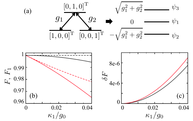
FIG. 1 (color online). (a) Mechanical dark mode. (b) F (solid) and F_1 (dashed) for |\alpha| = 1 (upper curves) and |\alpha| = 1, r = 0.4 (lower curves). (c) \delta F for |\alpha| = 1 (lower curve) and |\alpha| = 1, r = 0.4 (upper curve). Other parameters are \kappa_2 = 0 , g_1 = 5 \sin(t) , g_2 = -5 \cos(t) , and T = \pi/2 in arbitrary units.
