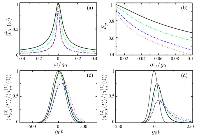
FIG. 2 (color online). (a) |\hat{T}_{31}(\omega)| , (b) F_p , and (c), (d) \langle a_{out}^{(2)}(t) \rangle / \langle a_{in}^{(1)}(0) \rangle for \sigma_\omega/g_0 = 0.008, 0.04 , respectively, with (\kappa_1, \kappa_2)/g_0 being (0.096, 0.054) (solid), (0.064, 0.036) (dash-dotted), (0.032, 0.018) (dotted), and (0.0192, 0.032) (dashed). Other parameters are \gamma_m/g_0 = 0.0002 , g_1 = 4 , and g_2 = 3 in arbitrary units.
