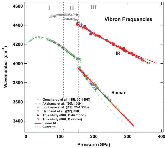
FIG. 2 (color). Low-temperature vibron frequencies as a function of pressure, including results from the present study as well as IR data from Refs. [18,27], and Raman data from Refs. [18,19]. Different symbols correspond to different experiments. The red lines are our fits of these combined IR and Raman vibron shift datasets. The blue dashed line is the Raman shift reported in Ref. [20], which follows a trend not found in the other studies.
