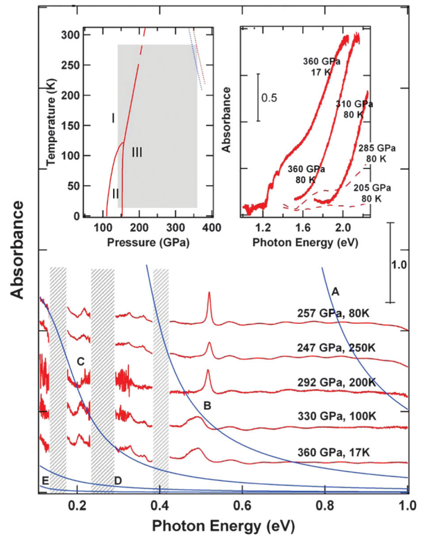
FIG. 3 (color). Absorption spectra at selected pressures and temperatures. Synchrotron IR spectra (red lines, offset for clarity) show the persistence of the vibron over the range of conditions studied. The blocked areas at low energy are regions of intrinsic and impurity absorption of the diamond anvils. The initial (160 GPa) sample thickness d for the top three spectra was 3.7 \mu\text{m} [corresponding to Fig. 1(a)], and for the lower two spectra d = 2.6 \mu\text{m} [Fig. 1(b)]. The blue lines are representative optical conductivities calculated assuming simple Drude model parameters (see Ref. [8]) to provide upper bounds on the possible carrier density: (A) \hbar\omega_p = 2 \text{ eV} , \hbar/\tau = 0.1 \text{ eV} ; (B) \hbar\omega_p = 1 \text{ eV} , \hbar/\tau = 0.1 \text{ eV} ; (C) \hbar\omega_p = 0.5 \text{ eV} , \hbar/\tau = 0.1 \text{ eV} . (D) \hbar\omega_p = 0.2 \text{ eV} , \hbar/\tau = 0.1 \text{ eV} ; (E) \hbar\omega_p = 0.2 \text{ eV} , \hbar/\tau = 0.01 \text{ eV} [28]. A sample thickness d = 2 \mu\text{m} was assumed. Curves D and E are consistent with the measured data. Sharp features at low energies arise from phonons and hydrogen-diamond interactions and are discussed elsewhere [8,9,28]. Left inset: Phase diagram showing the nominal P - T region explored (shaded area). The solid lines are I-II-III phase boundaries [6,11]; the dashed line is the extrapolation of the previously determined I-III phase line [11]. The blue and red dotted lines at higher pressures are predicted melting and plasma phase transition lines, respectively (see Refs. [17,25]). Right inset: Selected visible absorption spectra. The dashed red lines are from Ref. [18] and are rescaled to fit the plot. The absorption edge appears to have a weak temperature shift under these conditions, but only a limited P - T range has been explored [28].
