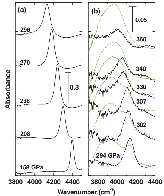
FIG. 1 (color). Representative synchrotron IR spectra of hydrogen in the region of the vibron ( \text{H}_2 stretching mode) at selected pressures and 80 K. (a) Spectra from an experiment reaching 300 GPa. (b) Spectra from a higher pressure experiment. Below 150 GPa (in phase I), and at room temperature and at higher pressures (in phase I), the vibron intensity is approximately 3 orders of magnitude lower than at higher pressures and <100 \text{ K} (phase III). Thus, single-channel transmission spectra measured under these conditions can be used as a reference (or background) spectrum to obtain clear signatures of the vibron. For (a) the single-channel spectrum measured at 140 GPa and 300 K was used as the reference. For the absorption spectra shown in green in (b), a single-channel transmission spectrum measured at 142 GPa and 300 K was used as the reference (see Ref. [28]). In order to ratio out the diamond phonon absorption band at these higher pressures, a series of single-channel transmission spectra measured at corresponding pressures and \geq 250 \text{ K} were also used as reference spectra to determine the absorption, as shown by the black curves in (b). The absorbance bar refers to the amplitude of these spectra; the absorbances for spectra in green are scaled by \frac{1}{2} in the plot. As a cross-check, peak positions were also determined using direct deconvolution of spectra having overlapping bands; the peak positions of the vibrons determined by both approaches were found to be within \pm 10 \text{ cm}^{-1} . Further details are provided in Ref. [28].
