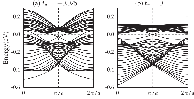
FIG. 2. One-dimensional energy bands for armchair strip in the (a) NI phase with t_n = -0.075 and (b) TI phase with t_n = 0 .
