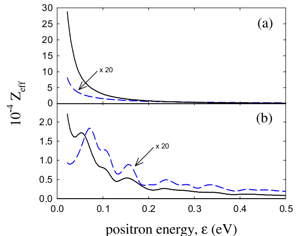
FIG. 3 (color online). SMRA contribution Z_{\text{eff}}^{(\text{stat})} , Eq. (3), convolved with the experimental beam distribution, for (a) chloroform ( \text{CHCl}_3 ) and (b) methyl chloride ( \text{CH}_3\text{Cl} ), when artificially changing the binding energy from 20 meV (dashed line) to 200 meV (solid line).
