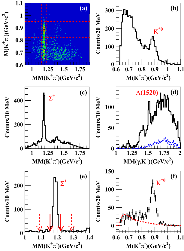
FIG. 1 (color online). (a) Scatter plot of the missing mass of the K^+ \pi^- system versus the invariant mass of the K^+ \pi^- system; (b),(c) projected spectra for the invariant mass and missing mass distributions, respectively; (d) missing mass of the K^+ (with a \pi^- detected), and the lower dashed histogram indicates the final even selection within 3\sigma of the \Sigma^+ peak and the K^{*0} peak; (e) missing mass distribution with solid arrows around the signal region ( K^{*0} peak) and dashed arrows showing the outside of the sideband regions; (f) same as (b), but with a cut on the \Sigma^+ peak after the sideband background subtraction, and the overlaid dashed line shows the estimated Y^* background.
