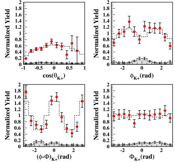
FIG. 2 (color online). Decay angular distributions of \cos\theta_{K^+} , \phi_{K^+} , (\phi - \Phi)_{K^+} , and \Phi_{K^+} in the GJ frame for the sum of vertical polarization and horizontal polarization after acceptance correction. The dotted lines show Monte Carlo data using the measured spin-density matrix elements, while the overlaid black histograms indicate the Y^* background yield from a Monte Carlo simulation.
