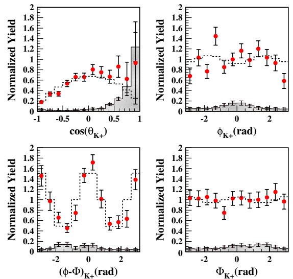
FIG. 3 (color online). Decay angular distributions in the helicity frame. Notations are the same as in Fig. 2.
