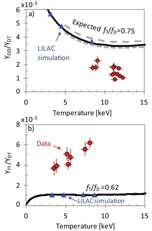
FIG. 3 (color online). (a) Measured Y_{dd}/Y_{dt} yield ratios as a function of ion temperature (red points). The solid line represents the expected yield ratio calculated using Eq. (6) for the average initial DT fuel mixture ( f_T/f_D \approx 0.75 ) used in this study. The grey dashed lines show the variation in the initial f_T/f_D due to tritium decay between these shots, which were obtained over a two-year period. 1D hydrodynamic simulations using LILAC (blue triangles) are also shown (for constant f_T/f_D \approx 0.75 ). The results show a suppression of the Y_{dd}/Y_{dt} yield ratio, indicating a lower deuterium fraction in the core than expected. (b) Measured Y_{tt}/Y_{dt} reaction yield ratios as a function of ion temperature (red points). The solid line represents the expected yield ratio for the ( f_T/f_D \approx 0.62 ) DT fuel mixture used in this study. The anomalously high Y_{tt}/Y_{dt} is consistent with a lower deuterium fraction in the core than expected, as suggested by the results in Fig. 3(a).
