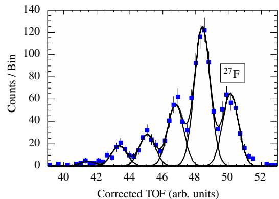
FIG. 1 (color online). Corrected TOF for fluorine isotopes produced from ^{29}\text{Ne} .
