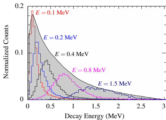
FIG. 2 (color online). Simulated resolution and acceptance of the experimental setup. Each colored histogram was generated by simulating a ^{28}\text{F} breakup at the indicated relative energy and then folding in detector resolution and acceptance cuts. The shaded curve was generated by simulating a ^{28}\text{F} breakup with the relative energy uniformly distributed from 0–3 MeV and folding in acceptance and resolution. The colored histograms are all normalized to a total area of unity, and the shaded curve was arbitrarily scaled to fit within the same panel.
