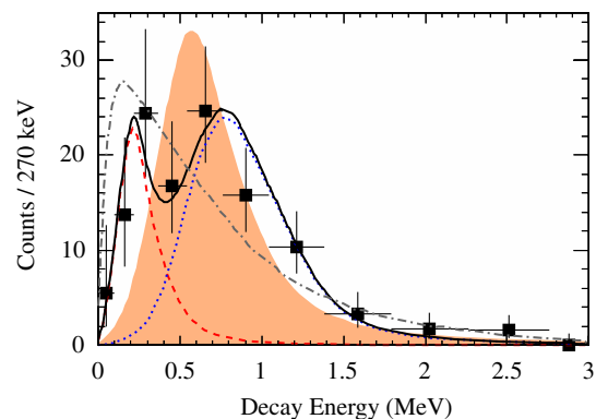
FIG. 3 (color online). Measured decay energy spectrum (including smearing from experimental resolution and acceptance) for ^{27}\text{F} + n coincidences. The filled squares with error bars are the measured data, and the dashed red and dotted blue curves represent the 220 and 810 keV simulation results, respectively. The solid black curve is the sum of the two resonances, with the ratio of 220 keV resonance to the total area being 28%. The filled orange curve is a simulation of a single resonance at 590 keV, and the gray dot-dashed curve is the best fit of a single s wave ( a_s = -0.05 fm).
