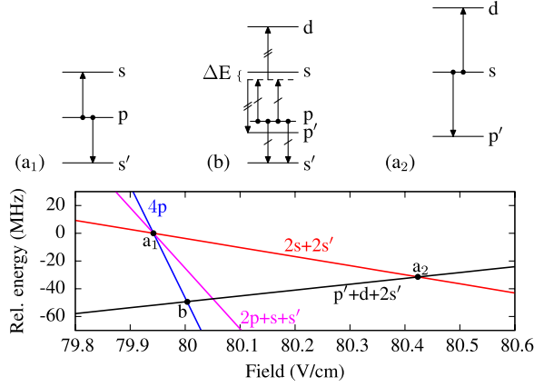
FIG. 1 (color online). Calculated four-atom energy for the two relevant 2-body resonances ( a_1 ) and ( a_2 ) and the p \rightarrow d 4-body resonance (b) as a function of the electric field.
