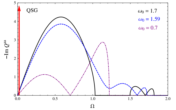
FIG. 3 (color online). rf spectral response function of the atomic qubits in the \text{QSG} phase for various photon frequencies and t^2 = 0.175 , g^2 = 0.05 , \Delta = 1 . The red arrow at \Omega = 0 illustrates the delta function contribution with weight q \sim q_{\text{QSG}} from Eqs. (12) and (14).
