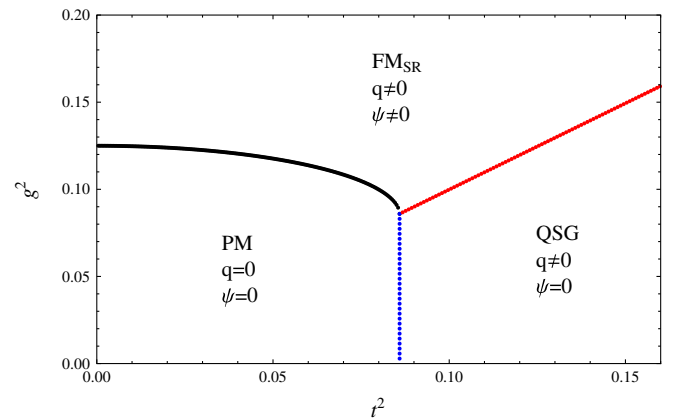
FIG. 1 (color online). Zero-temperature phase diagram for \omega_0 = 1, \Delta = 1 computed from Eq. (11). PM means paramagnet, FM SR superradiant ferromagnet, and QSG quantum spin-glass. q is the Edwards-Anderson order parameter and \psi is the atomic population inversion or ferromagnetic order parameter.
