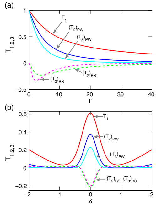
FIG. 3 (color online). Many-body bound-state effect causing photon blockade. (a) Transmission as a function of the decay rate \Gamma into the waveguide modes for \Omega = 1.6 . The presence of the many-body bound states suppresses the multiphoton transmission. (b) Transmission as a function of incident photon detuning \delta for \Gamma = 6 and \Omega = 1.6 . The bound states strikingly oppose multiphoton EIT; off resonance, their constructive interference produces photon-induced tunneling.
