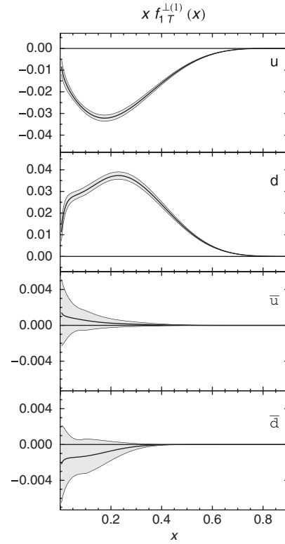
FIG. 1. The function x f_{1T}^{\perp(1)a}(x; Q_0^2) (see text) as a function of x at the scale Q_0 = 1 GeV for a = u, d, \bar{u}, \bar{d} from top panel to bottom, respectively. The uncertainty bands are produced by the statistical errors on the fit parameters listed in Table I.
