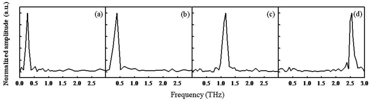
FIG. 5. The spectra of THz radiation for time delay \tau = 0.4 ps (a), 0.7 ps (b), 1.8 ps (c), and 3.6 ps (d).
