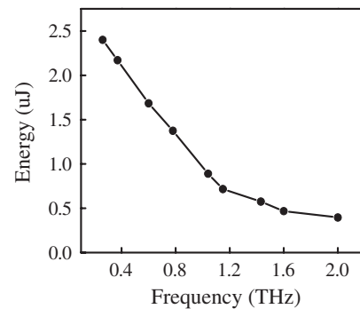
FIG. 7. THz pulse energy as a function of radiation frequency.
