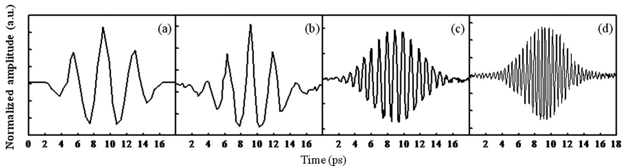
FIG. 4. Measured field autocorrelation of THz radiation for time delay \tau = 0.4 ps (a), 0.7 ps (b), 1.8 ps (c), and 3.6 ps (d). The spectra of THz radiation for time delay \tau = 0.4 ps (a), 0.7 ps (b), 1.8 ps (c), and 3.6 ps (d).
