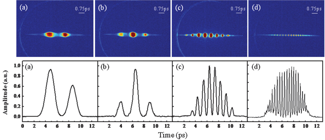
FIG. 3 (color). Measured longitudinal distribution (top row) and projected electron density distribution (bottom row) for a temporally modulated electron bunch.
