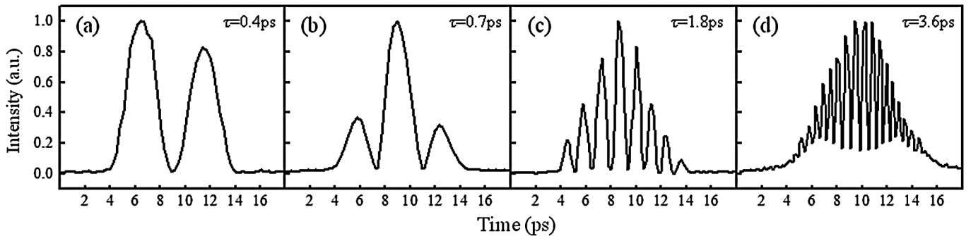
FIG. 2. Temporal profiles of the photocathode drive laser pulses for different time delays.
