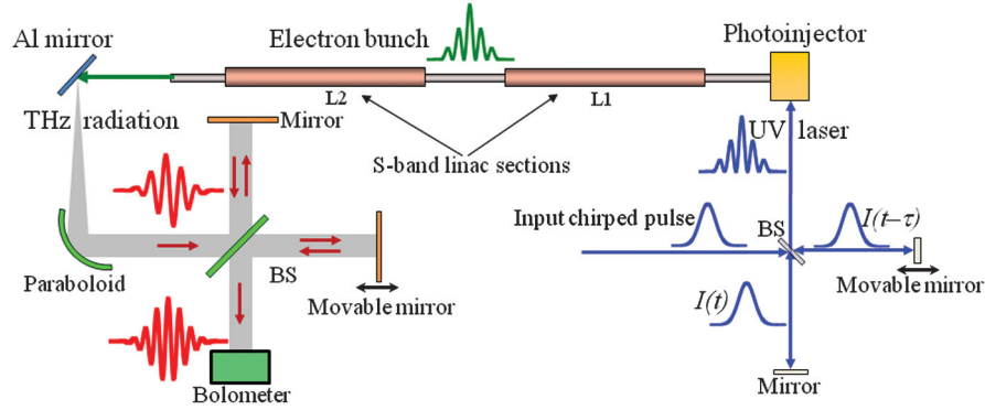
FIG. 1 (color). Schematic of a linac-based light source for tunable THz generation and characterization.
