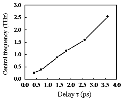
FIG. 6. Variation of THz frequency as a function of time delay \tau .
