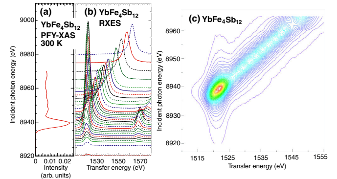
FIG. 2 (color online). (a) and (b) RXES spectra as a function of the incident photon energies with PFY-XAS spectra at 300 K for \text{YbFe}_4\text{Sb}_{12} . The vertical offset of the RXES spectra in panel (b) corresponds to the incident energy in the PFY-XAS spectrum at which they were measured in panel (a). The energy transfer is the difference between the incident and emitted photon energies. (c) Contour image of the RXES spectra.
