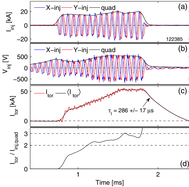
FIG. 4 (color online). X - and Y -injector currents (a) and voltages (b) with quadrature values; (c) toroidal current and toroidal current time-averaged over an injector cycle. The current decay time \tau_I = -I/(dI/dt) is averaged over 100 \mu\text{s} after the injectors are off; (d) current amplification of the time-averaged signals.
