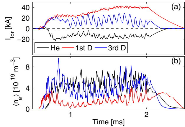
FIG. 2 (color online). (a) The toroidal currents and (b) line-averaged electron densities of a helium shot (121959) and subsequent deuterium shots (121961 and 121963).
