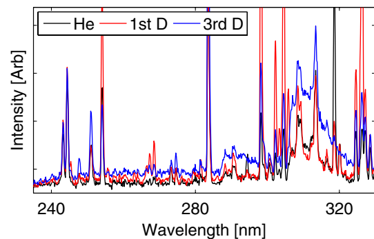
FIG. 3 (color online). Line radiation of a helium shot (121959) and subsequent deuterium shots (121961 and 121963).
