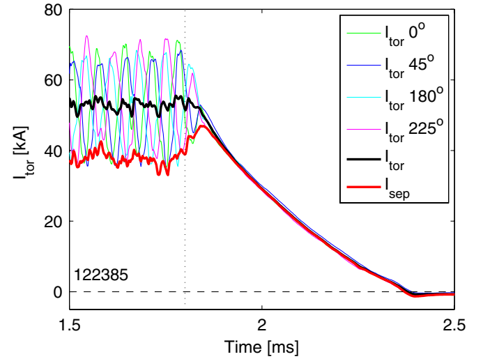
FIG. 5 (color online). Toroidal current measurements at the four toroidal locations with the average toroidal current and the separatrix current. The vertical dotted line at 1.8 ms indicates the time when the injectors are turned off.
