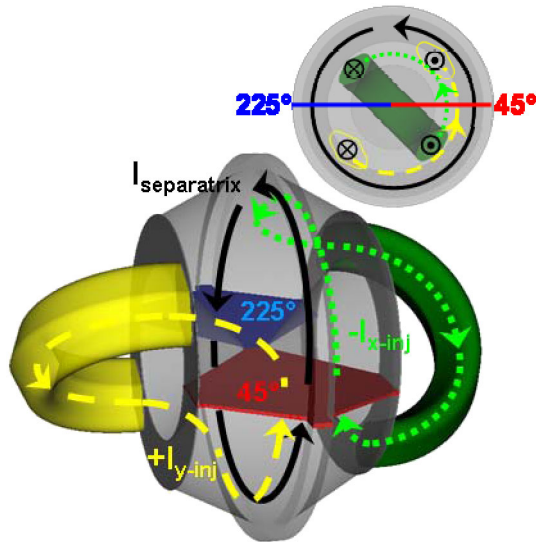
FIG. 1 (color online). The HIT-SI geometry is shown with the confinement volume in the center, the Y injector to the left, and the X injector to the right. The poloidal cross sections at 45° and 225° are shaded. Included in the figure is a model representing the current paths in HIT-SI. The separatrix current (solid line) is shown with the injector currents at a time with negative X-injector (dotted line) and positive Y-injector (dashed line) current. In the top right of the figure is a 2D projection of the current paths with the view looking at the X injector from the midplane of the confinement volume. At the representative time shown the X injector, Y injector, and separatrix current pass the 45° plane, while only the separatrix current passes the 225° plane.
