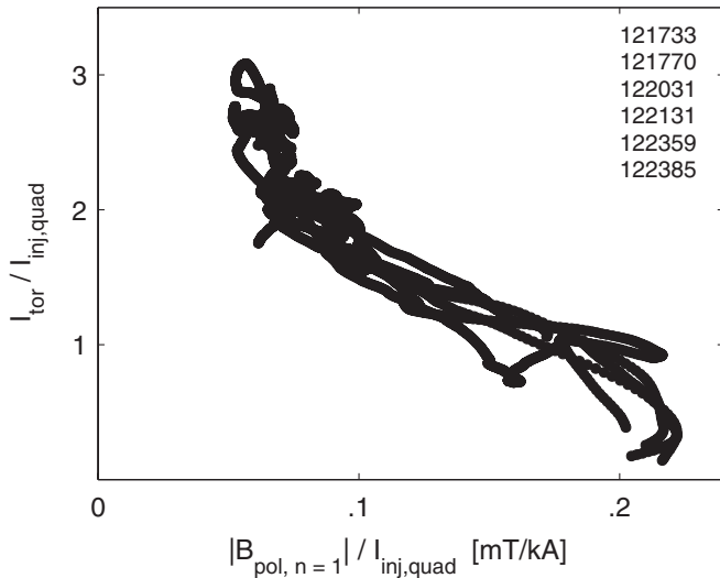
FIG. 7. Scatter plot of the current amplification compared to the magnitude of the n = 1 toroidal mode of the poloidal magnetic field averaged over an injector cycle and normalized by the quadrature injector signal for six shots.
