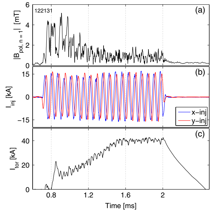
FIG. 6 (color online). (a) The magnitude of the n = 1 toroidal Fourier mode of the poloidal magnetic field, (b) the injector currents, and (c) the toroidal current.
