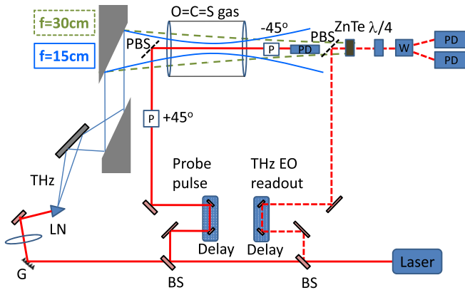
FIG. 1 (color online). Schematic representation of the two setups used in this work. An optical pulse was used to generate the single-cycle THz pulse that was passed through the gas cell to induce coherent rotational motion. Either the THz electro-optic (EO) readout pulse was generated for the measurement of the periodic FID emission owing to the induced molecular orientation, or the optical probe pulse was generated for measurement of the THz-induced birefringence due to molecular alignment. For the FID (birefringence) measurements the THz beam (FWHM \sim 1.5 cm) was focused by f = 30 cm ( f = 15 cm) off axis parabolic reflectors to create the dashed green (solid blue) THz spatial distributions, respectively. G, grating; LN, lithium niobate THz generation crystal; BS, beam splitter; P, polarizer; W, Wollaston prism; PD, photodetector; PBS, Pellicle beam splitter. (In order to switch between the two setups, we replace the last parabolic reflector and remove the first Pellicle, the -45^\circ P and the single PD).
