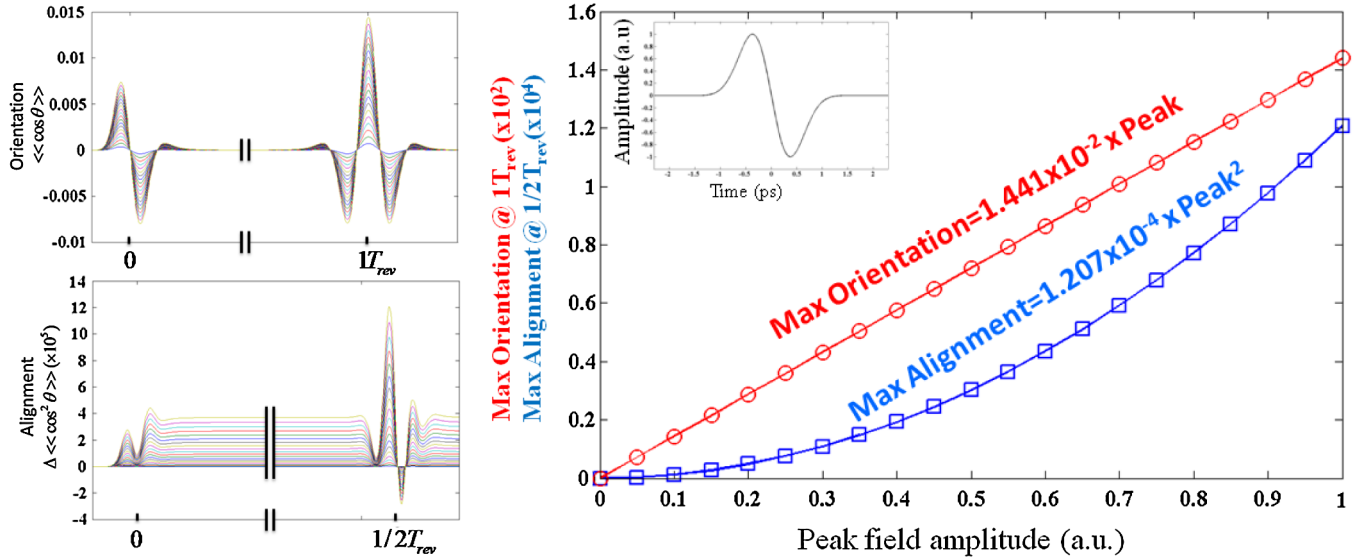
FIG. 3 (color online). (a) Time-dependent orientation and alignment induced in OCS at 300 K, calculated for a series of amplitudes of the driving field profile depicted in the inset of panel b . (b) By fitting the peak orientation and peak alignment we get their peak amplitude dependences on the driving field, as marked in the figure.
