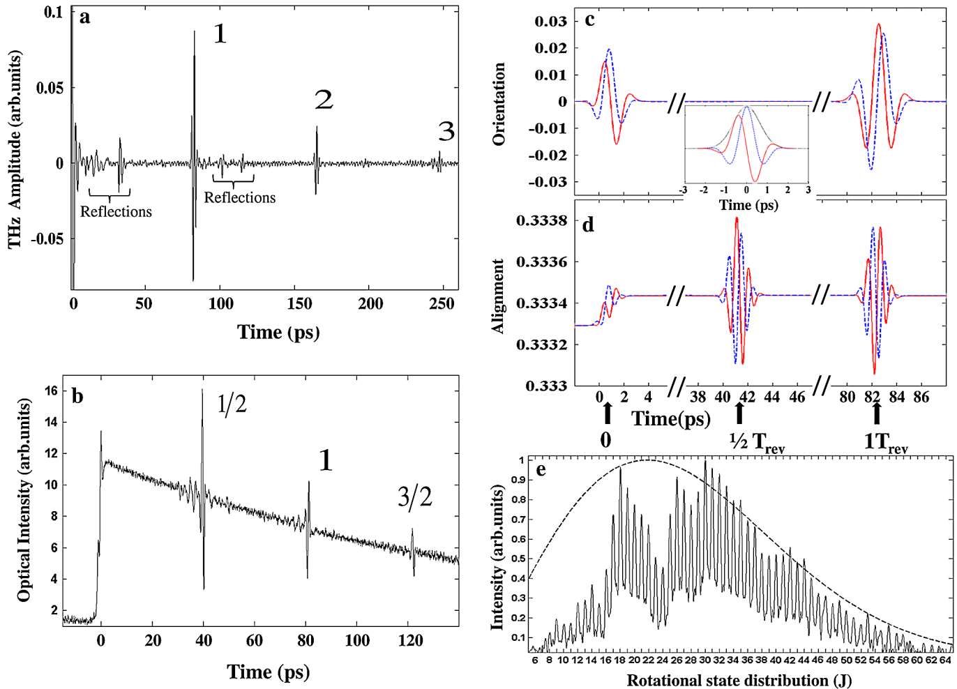
FIG. 2 (color online). (a) Electro-optic sampling of the FID emission from the OCS gas cell following the THz pulse. (b) Alignment-induced birefringence in 350 torr OCS at 300 K. (c) Numerical simulation results for orientation \langle\langle\cos\theta\rangle\rangle(t) induced by a single-cycle THz pulse. Two simulations are shown for THz pulses with the same pulse envelope (inset, black dotted curve) and with fields phase-shifted by 90^\circ (inset, solid red and dashed blue curves). (d) Numerical simulation results for alignment \langle\langle\cos^2\theta\rangle\rangle(t) induced by a single-cycle THz pulse. Simulations are shown for the same phase-shifted THz waveforms as in (c) and for OCS gas at 300 K. (e) Normalized rotational level ( J state) contribution to the coherent signal shown in (b). The calculated thermal rotational distribution at 300 K is depicted by the dashed curve.
