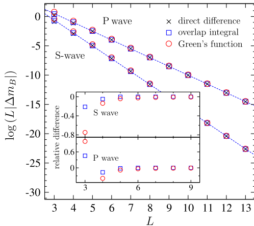
FIG. 2 (color online). S - and P -wave mass shifts \log(L|\Delta m_B|) as functions of the box size L (in lattice units). We show the results obtained from the direct difference Eq. (2) (crosses), evaluation of the overlap integral Eq. (3) (squares), and discretized versions of Eqs. (6) and (8) (circles). The dashed lines are linear fits to the squares. In the inset, we show the relative difference between the direct results and the overlap (squares) and Green's function (circles) data.
