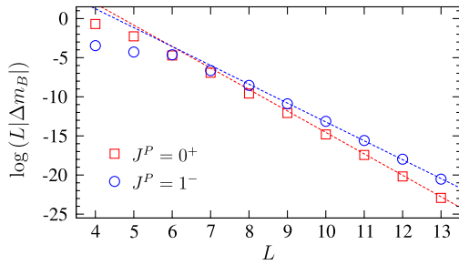
FIG. 3 (color online). Trimer mass shifts \log(-L|\Delta m_B|) as functions of the box size L (in lattice units). We show lattice results for the two lowest-lying trimer states with J^P = 0^+ (squares) and J^P = 1^- (circles).
