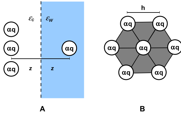
FIG. 2 (color online). Hexagon of images at the surface. In (A) the side view. In (B) the self-image and the nearest neighbors.
