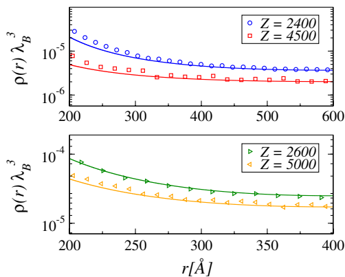
FIG. 4 (color online). Density profiles in the far-field. Symbols represent the simulation data and lines are the predictions of the present theory. The parameters are the same as in Fig. 3.
