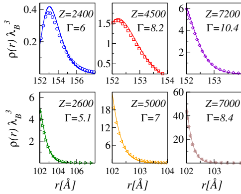
FIG. 3 (color online). Density profiles near the colloidal surface. Symbols are the simulation data and lines are the predictions of the present theory. Circles, squares and diamonds are simulation data for \alpha = 3 , a = 150 Å and R = 600 Å. Right, left triangles and stars are simulation data for \alpha = 2 , a = 100 Å and R = 400 Å. The ionic radius is r_c = 2 Å.
