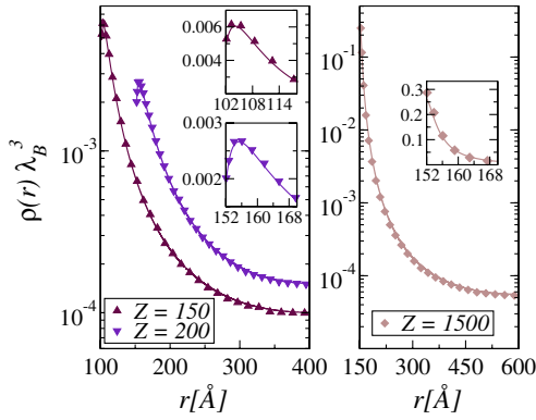
FIG. 1 (color online). Density profiles of monovalent counterions. Symbols represent simulation data and lines represent the modified PB theory. The parameters of the simulations are \alpha = 1 , r_c = 2 Å; down triangles ( a = 150 Å and R = 400 Å); up triangles ( a = 100 Å and R = 400 Å); diamonds ( a = 150 Å and R = 600 Å). The insets show the profiles close to the colloidal surface.
