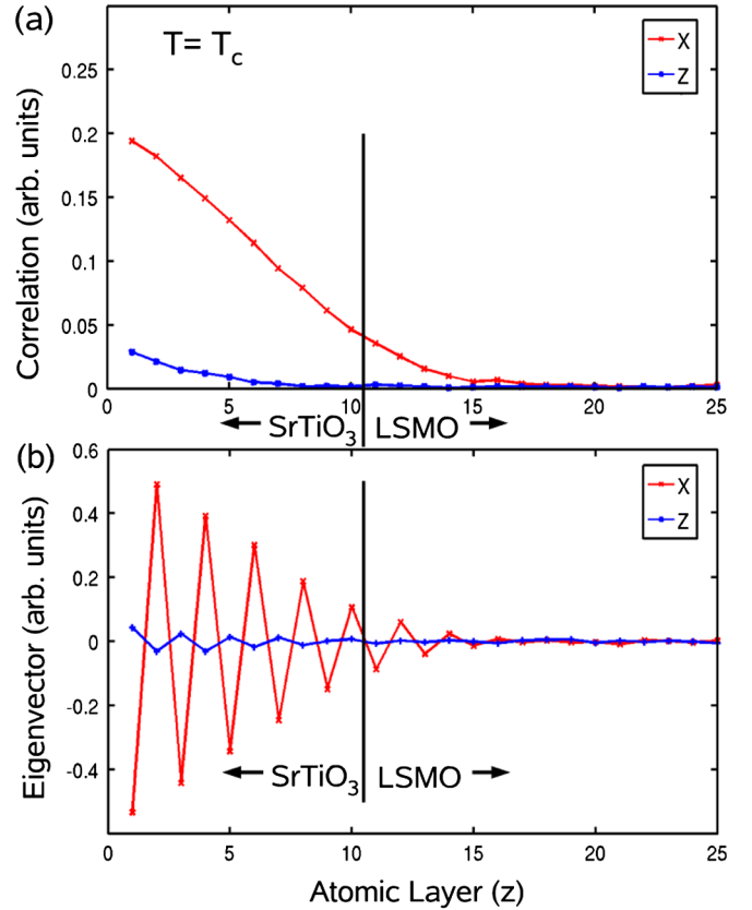
FIG. 3 (color online). Density functional theory and Monte Carlo results of phonon transfer from STO to LSMO. (a) Absolute magnitude of the correlation function of oxygen displacements with those deep in the STO as a function of layer number at T = T_c . x and z indicate displacements stemming from octahedral rotation around the x and z axis, respectively. (The y component is equal to x by symmetry.) (b) x and z components of the lowest frequency eigenvector at T = T_c . The layer-to-layer sign changes reflect the AFD nature of the oxygen displacements.
