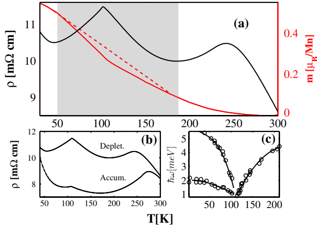
FIG. 1 (color online). Enhanced carrier-phonon scattering. (a) Left axis: Resistivity of an 11 uc \text{La}_{0.53}\text{Sr}_{0.47}\text{MnO}_3 film showing a strong cusp at 108 K. The PZT overlayer is in the depletion state. Right axis: Magnetic moment of a 15 uc \text{La}_{0.55}\text{Sr}_{0.45}\text{MnO}_3 film. The moment is measured along the [100] direction under an applied magnetic field of 1 kOe. A dip in the moment is observed, overlapping the temperature range of the resistivity cusp (emphasized by the gray box). The dashed line is a linear interpolation between the edges of the dip region. (b) The resistivity of the 11 uc film for the two polarization states of the PZT layer. (c) Energy of the \Gamma_{25} phonon mode in STO, showing the softening around the STO transition temperature (after Ref. [10]). Lines are a guide to the eye. Below the structural phase transition temperature the mode splits due to the breaking of cubic symmetry.
