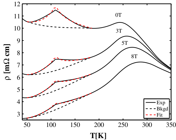
FIG. 4 (color online). Resistivity of an 11 uc film of \text{La}_{0.53}\text{Sr}_{0.47}\text{MnO}_3 as a function of temperature, for several out-of-plane magnetic field values. The PZT overlayer is in the depletion state. Black dashed lines are interpolations excluding the cusp, and the gray (red) dashed lines are fits to \Gamma_{25} phonon coupling.
