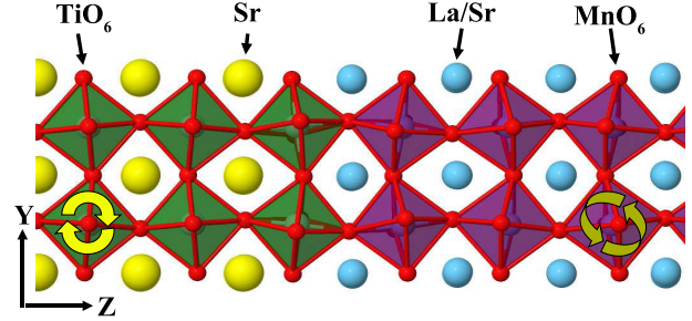
FIG. 2 (color online). Side view of the STO-LSMO interface geometry. The plot shows calculated ground-state atomic positions. Away from the interface, the STO is fixed to have bulklike octahedral rotations around the x axis (into the page). The LSMO geometry at the interface is modified by the STO; however, the LSMO relaxes to its bulklike octahedral rotations around both in-plane axes within 2–3 unit cells.
