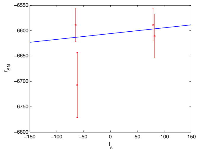
FIG. 1 (color online). Fitting r_{NS} to r_{NS} = r_{NS}^A + r_{NS}^{GR} = \kappa_{NS} f_s + \lambda_{NS} + r_{NS}^{GR} .
