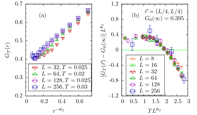
FIG. 2 (color online). (a) Correlation functions at low temperatures for L = 32, 64, 128, 256 plotted versus r^{-\theta_s} , using \theta_s = 0.50 . Droplet theory based on the entropy of the droplets predicts a linear curve at small values of r^{-\theta_s} and large L , as is seen. (b) Sample scaling collapse for correlation function G_T(\vec{r}) . Using nonzero-temperature scaling, we expect L^{\theta_s} [G_T(\vec{r}) - G_0(\infty)] \approx g(\vec{r}/L, TL^{\theta_s}) . Adjusting G_0(\infty) for the best collapse, we find G_0(\infty) = 0.395 \pm 0.010 .
