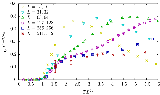
FIG. 3 (color online). Scaling plot for the low- T specific heat C . For T < L^{\theta_s} , there are no active droplets, so C is exponentially suppressed. The low- T scaling behavior in large-enough systems is seen when CT^{1-2/\theta_s} is flat at TL^{\theta_s} > 1 . The value [28] of \theta_s = 0.50 is independently set by the scaling of the entropy of domain walls.
