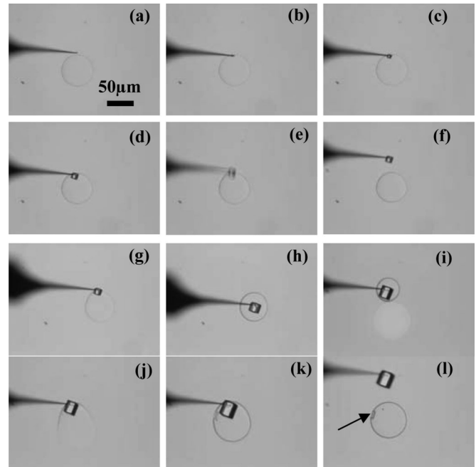
FIG. 4. Panels (a)–(l) represent a time sequence showing the nucleation and growth of NaCl at supersaturation \beta > 1.97 . (a) 0.7 M NaCl initial droplet size 56 \mu\text{m} ( \approx 51 \text{ pL} assuming a spherical shape for the droplet). All the micrographs are at the same magnification. See Supplemental Material [17] for a movie of this process.
