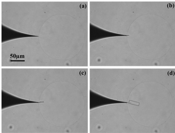
FIG. 3. Panels (a)–(d) represent a time sequence showing the nucleation and growth of KCl in DMS oil, initial condition: undersaturated KCl solution ( \beta = 0.5 ), (a) droplet size 147 \mu\text{m} ( \approx 1.66 \text{ nL} assuming a spherical shape for the droplet). All the micrographs are at the same magnification, the time between (b) and (d) is 1.3 s.
