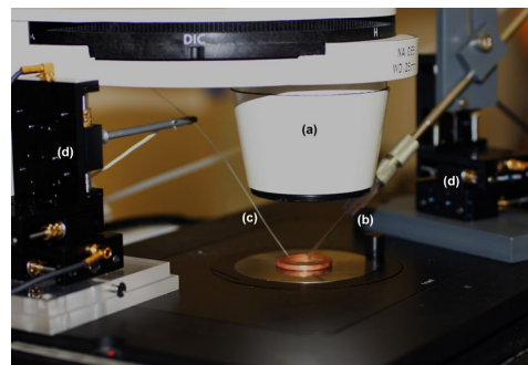
FIG. 1 (color online). Image of the whole experimental setup, (a) microscope, (b) glass capillary, (c) tungsten wire sharp tip, Supplemental Material [17] contains transmission electron micrographs of tungsten tips, and (d) XYZ miniature translation stages.
