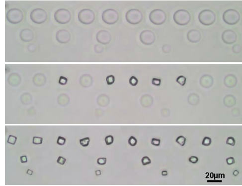
FIG. 2 (color online). Time sequence showing nucleation and fast growth of NaCl crystals. (a) At t = 0.45 s NaCl microdroplets of volumes ranging from 3 to 1 pL are generated (assuming a spherical shape for the droplet), (b) t = 4638 s, and (c) t = 6120 s. All the micrographs are at the same magnification.
