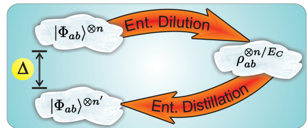
FIG. 1 (color online). Entanglement dilution-distillation cycle. The entanglement loss is given by \Delta . In the case of reversible entanglement, \Delta vanishes. In the irreversible case of Eqs. (8) and (9), \Delta is the regularized quantum discord.
