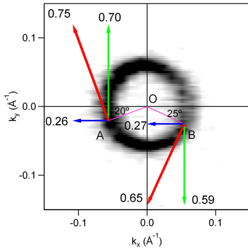
FIG. 4 (color online). Vector analysis of spin polarization in \text{Bi}_2\text{Se}_3 . The green (blue) arrows represent the spin polarization in the y ( x ) direction, determined from Fig. 3. The red arrows correspond to the total spin polarization. The lengths of the arrows indicate the magnitudes of spin polarizations. The origins of the arrows correspond to the k positions of points A and B . The intensity map represents the constant energy contour at -0.1 eV from spin-integrated ARPES data.
