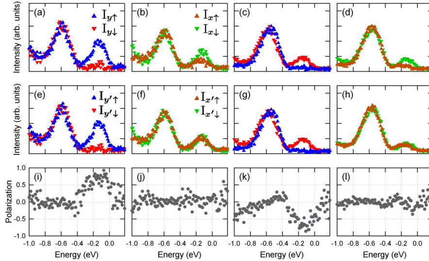
FIG. 3 (color online). The spin-resolved photoemission of the surface state of \text{Bi}_2\text{Se}_3 . (a)–(b) Spin-resolved spectra with the polarization vector along the y and x directions for point A from Fig. 2(a). (c)–(d) same for point B . (e)–(h) Spin-resolved spectra for points A and B with the polarization vectors along the red arrows in Fig. 4. The corresponding spin polarizations are shown in (i)–(l) All the spectra were measured at photon energy 50 eV at T = 77 K.
