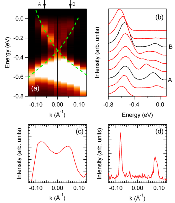
FIG. 2 (color online). Spin-integrated spectra of \text{Bi}_2\text{Se}_3 measured at 50 eV photon energy using the SARPES analyzer. (a) ARPES spectra along the momentum line \Gamma M near the center of the surface BZ, measured in steps of 0.5^\circ . The green line represents the surface state dispersion, extracted from momentum distribution curves (MDCs) from the ARPES spectrum shown in Fig. 1(b). A and B indicate the k positions where the spin-resolved measurements were performed. (b) energy distribution curves (EDCs) from (a). (c) MDC at the Fermi level from intensity contour in (a), interpolated to 4 times the number of original data points. (d) MDC from the Fermi surface map in Fig. 1(e) along the k_y = 0 line. The Lorentzian fit gives a full width at half maximum of 0.009 \text{ \AA}^{-1} , or 0.15^\circ .
