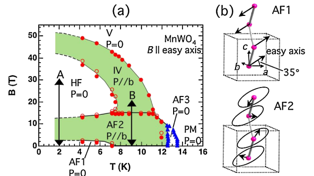
FIG. 2 (color online). (a) The magnetic phase diagram of MnWO 4 for B parallel to magnetic easy axis [13]. Ferroelectric phases are shaded in green. The present experiment has been performed along the arrows A and B. (b) A schematic diagram of the magnetic structures in the AF1 and AF2 phases. In AF1, the magnetic easy axis lies in the ac plane and is tilted by 35^\circ from the a axis.
