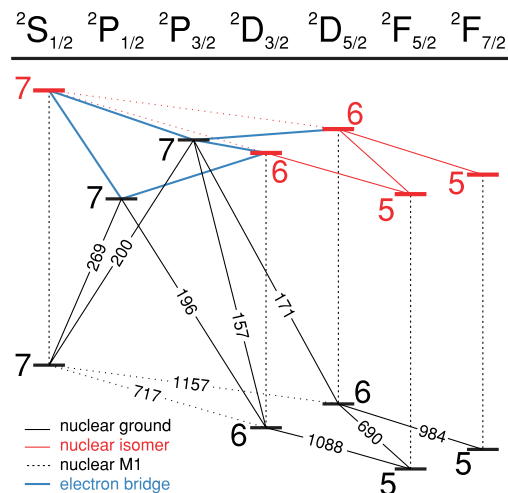
FIG. 1 (color online). A diagram of electronic energy levels and electric-dipole transitions including both nuclear ground and excited isomeric manifolds. Direct nuclear magnetic dipole ( M1 ) decay channels and electron-bridge pathways suitable for the isomer search are shown. Optical transition wavelengths are in nm and the integers near atomic levels indicate principle quantum numbers.
