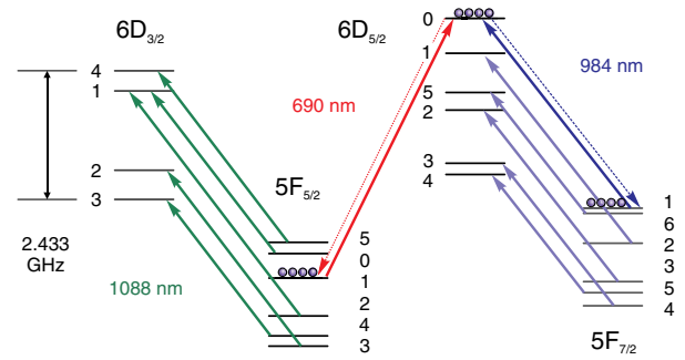
FIG. 3 (color online). Various optical transitions between hyperfine levels in ^{229}\text{Th}^{3+} employed during laser cooling. See text for details.
