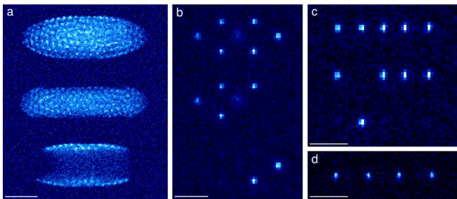
FIG. 4 (color online). Trapped ^{229}\text{Th}^{3+} and ^{232}\text{Th}^{3+} ions, laser cooled to crystallization. (a) Three successive images were taken of about 200 crystallized \text{Th}^{3+} ions. The top image was taken with both ^{229}\text{Th} and ^{232}\text{Th} 690 nm fields present. The ^{232}\text{Th} 690 nm field was then removed for the middle image. The ^{232}\text{Th} 690 nm field was then reintroduced and the ^{229}\text{Th} 690 nm field simultaneously removed for the bottom image. The larger mass-to-charge ratio of ^{232}\text{Th}^{3+} causes its radial accumulation in the outer shells of the crystal. The short focal depth of the imaging system is apparent as most of the ^{232}\text{Th}^{3+} shell is out of focus. The integration time is 1 s for all three images. (b),(c) The same imaging protocol used in (a) is used on smaller samples. The integration time is 2 s for all images. (d) A linear chain of four ^{229}\text{Th}^{3+} ions is shown. The integration time is 3 s. The scale bar in (a) is 500 \mu\text{m} and in (b)–(d) are 100 \mu\text{m} .
