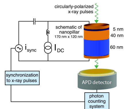
FIG. 1 (color online). Schematic of the experimental setup. The sample is positioned perpendicular to the incoming x-ray pulses and the transmitted x-ray intensity is recorded by an avalanche photodiode (APD) detector.
