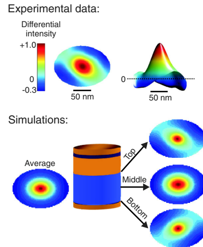
FIG. 3 (color online). Comparison of experimental data and micromagnetic simulation of the static magnetization distribution. Top: The magnetic contrast within the sample area of the magnetic image, Fig. 2(b), with pseudo color (left) and its surface plot (right), where the height is proportional to the out-of-plane magnetization. Bottom: Micromagnetic simulation, showing the out-of-plane component of the equilibrium magnetization in different planes of an isolated 60 nm-thick Py pillar with the same dimensions as in our sample (as shown).
