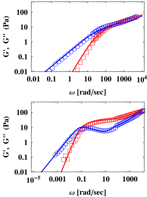
FIG. 2 (color online). Experimental data and theoretical comparisons for the storage modulus G'(\omega) (red squares) and the loss modulus G''(\omega) (blue circles) for two different suspensions of thermosensitive particles, as reported in [13]. The values of the parameters for the top and bottom panels, respectively, are \rho = 0.04, 3 \times 10^{-4} ; \nu^* = 0.001, 10^{-3}\rho ; \zeta = 1.0, 0.5 ; \bar{\Lambda} = 200, 40 ; \mu = 12, 35 Pa; and \tau_K = 0.004, 0.002 sec. In all cases, \zeta_1 = 1 and c = 0.1 .
