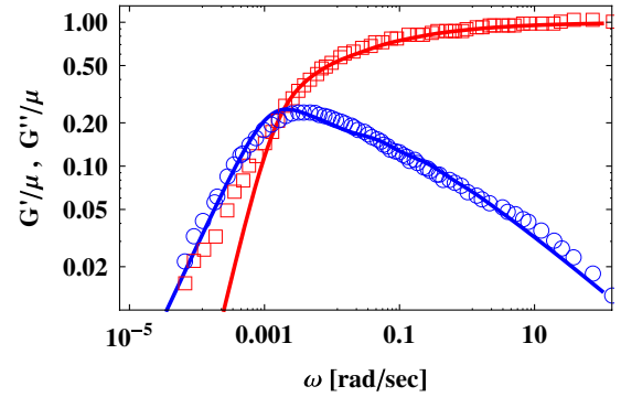
FIG. 1 (color online). Experimental data for Vitreloy 4 and theoretical comparisons for the storage modulus G'(\omega) (red squares) and the loss modulus G''(\omega) (blue circles). The data points were extracted from Fig. 2 in [1], where very similar curves for oxide and polymeric glasses can be found.
