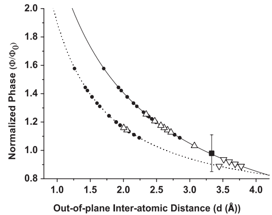
FIG. 3. Normalized phase of the exit wave as a function of out-of-plane interatomic distance for each individual atom column at the vacancy perimeter for the simulated and the TEAM I images in bilayer h -BN. The phase in the defect-free region of bilayer h -BN is normalized to unity. The two solid and dashed curves show the normalized phase versus the out-of-plane distance for a simulated B-N pair with no in-plane (solid line) and 35 pm in-plane (dashed line) distortion. Normalized phase for each individual atom column at the perimeter of the simulated boron ( \Delta ) and simulated nitrogen ( \nabla ) monovacancies is projected on the solid and dashed lines. The data points projected on the dashed line correspond to the vacancy edge atoms with in-plane distortion. TEAM I atom columns at the perimeter of the monovacancies ( \bullet ) are projected on both the solid and dashed lines, while TEAM I atom columns at the defect-free region ( \blacksquare ) are projected on the solid line. The error bar corresponds to 13% variation in the magnitude of the phase shift in the defect-free region of the film.
