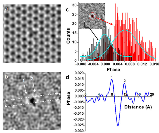
FIG. 4 (color online). (a) Phase of a monovacancy and (b) residual phase around the vacancy after the phase from the defect-free region is subtracted. (c) Distribution of residual phase showing a phase shift at the vicinity of the vacancy compared to the background. (d) Residual phase line profile across the vacancy previously shown in (b).
