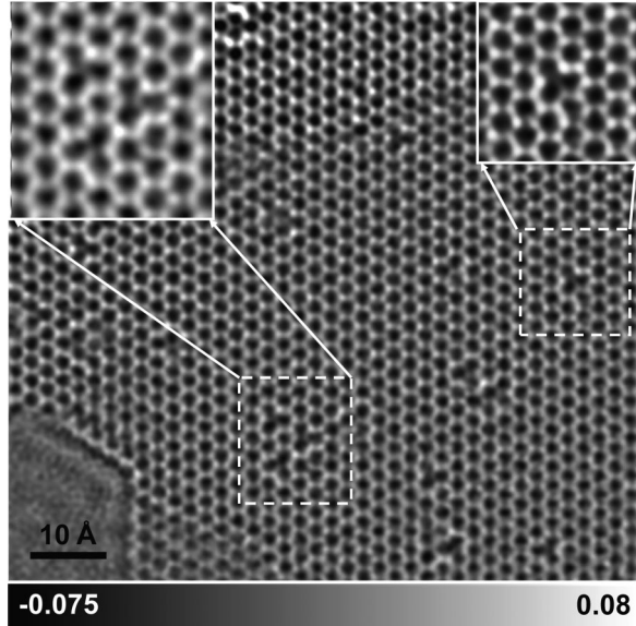
FIG. 1. Reconstructed phase of a bilayer h -BN imaged by the TEAM I microscope. The magnified inset images show broken symmetry at the defect sites. Color bar shows the relative phase in radians.
