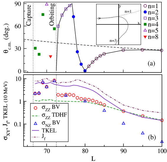
FIG. 1 (color online). (a) Scattering angle as a function of angular momentum L in units of \hbar for ^{40}\text{Ca} + ^{40}\text{Ca} at E_{c.m.} = 128 MeV. n is the number of times the x (collision axis) or y axis has been crossed by the fragment. The solid line is to guide the eye. The dashed line corresponds to Rutherford trajectories. The inset gives examples of trajectories for n = 1 and 3. (b) TDHF (dashed line) and BV (circles) fluctuations of Z , BV correlations between N and Z (triangles), and intrinsic angular momentum J_f of the outgoing fragments (dot-dashed line). The TKEL (solid line) is given in units of 10 MeV. The vertical dotted lines show the range of L leading to orbiting or capture trajectories.
