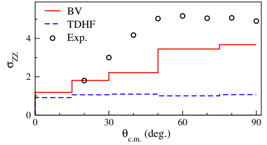
FIG. 2 (color online). Comparison between BV (solid line) and TDHF (dashed line) predictions of \sigma_{ZZ} for damped events (see text) as a function of \theta_{c.m.} with data (circles) from [24].
