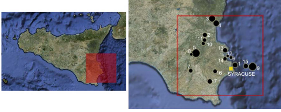
FIG. 2 (color online). Map of Sicily showing the location of the monitored site (yellow square) and epicenters (black circles) of nearby earthquakes (listed in Table I) that occurred during the monitoring period.
