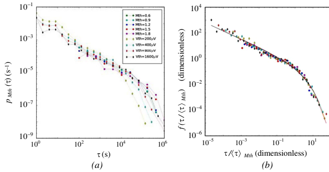
FIG. 5 (color online). Waiting-time PDFs for five seismic magnitude thresholds M_{th} and four AE signal thresholds V_{th} (a) and their collapse onto a single curve illustrating the fulfillment of a common scaling law (b).
