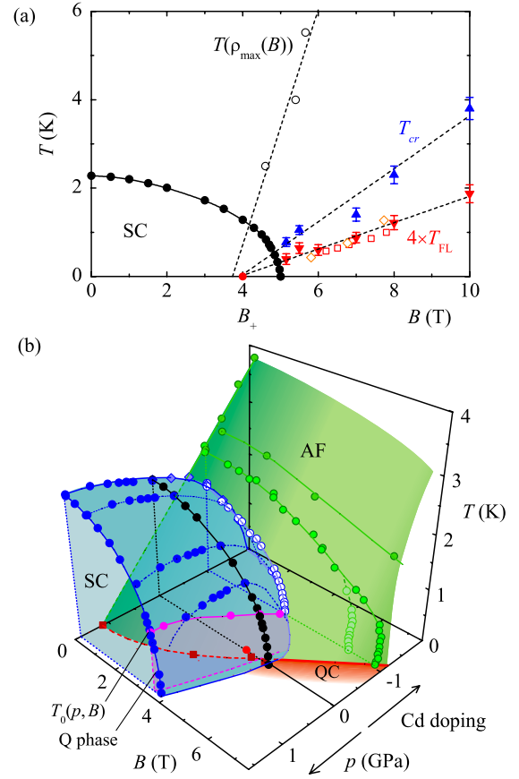
FIG. 3 (color online). (a) The (B, T) phase diagram of CeCoIn 5 at ambient pressure constructed from our measurements of the superconducting transition (black dots), the onset of FL behavior at T_{FL} , and the change in the critical behavior at T_{cr} . In addition, literature data are shown for the maximum of the magnetoresistance T[\rho_{\max}(B)] [26] and T_{FL} determined by Hall effect (open squares [25]) and resistivity measurements (open diamonds [24]). (b) Tentative (p, B, T) phase diagram of CeCoIn 5 . The data from (a) have been extended by published measurements under hydrostatic (solid [blue] dots [14,28–30]) and under negative, chemical pressure on CeCoIn 5-x Cd x (solid [green] [ T_N ] and open [blue] [ T_c ] circles [31–33]). To account for the different sample qualities and varying T_c definitions the measurements have been scaled to match in the regions of overlap. B_+ (solid [red] dot), and the onset of the NFL behavior (solid [dark red] squares [14]) are projected onto the T = 0 plane.
