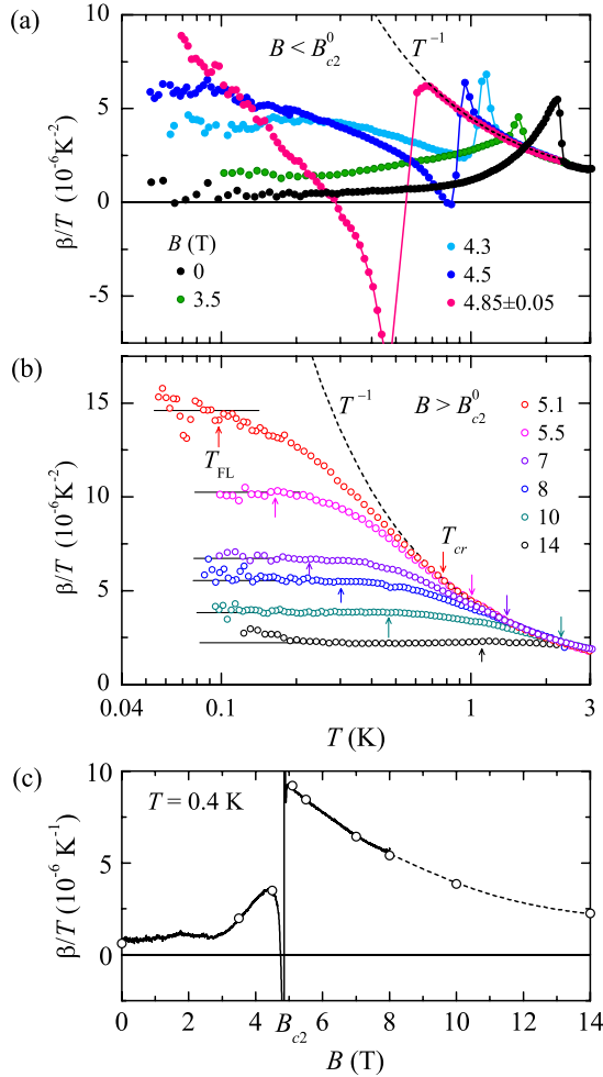
FIG. 1 (color online). The volume thermal-expansion coefficient of CeCoIn 5 divided by temperature \beta/T in magnetic fields parallel to the c axis below (a) and above B_{c2}^0 (b). In order to optimize the resolution of the experiment, different samples were used to measure \alpha_a and \alpha_c . They have slightly different B_{c2}^0 values of \approx 5.1 T and \approx 5.05 T, respectively. Therefore, the data for B = 4.85 T are a combination of measurements at B = 4.8 T and 4.9 T where the T_c values are identical. The dashed lines represent the non-Fermi-liquid behavior for the HMM model. (c) \beta/T as a function of B at T = 0.4 K obtained from magnetostriction measurements (continuous line) and from temperature-dependent measurements at constant B (circles). Dashed line is a guide to the eye.
