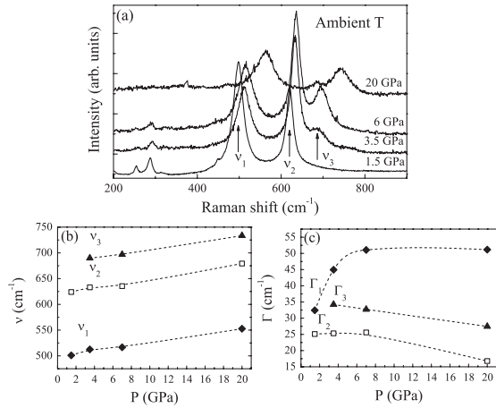
FIG. 1. (a) High P Raman spectra collected at ambient T . (b) Pressure dependence of the main phonon peak frequencies. (c) Pressure dependence of peak widths. Dashed lines are guides for the eye.
