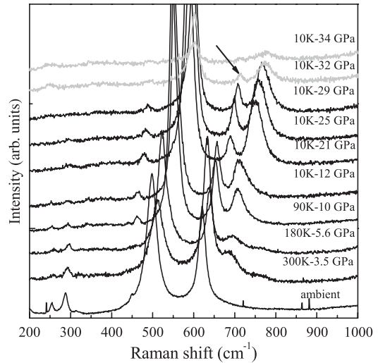
FIG. 2. Raman spectra for \text{LaMnO}_3 collected as a function of P and T . The gray spectra were collected when \text{LaMnO}_3 enters metallic state. The black arrow indicates the \nu_2 peak that is still observed at 32 GPa.
