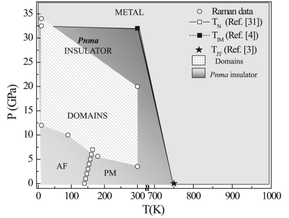
FIG. 4. P - T phase diagram. Paramagnetic phase (PM), antiferromagnetic phase (AFM). Gray dashed area and white circles frame the P - T region with coexistence of domains. P - T evolution of T_N (white squares) [31]. The star and the black square indicate the JT transition and the IMT temperatures, respectively [3,4]. Dark gray area indicates the insulating P - T region. The light gray color is used for the P - T region of the phase diagram which has been poorly explored.
