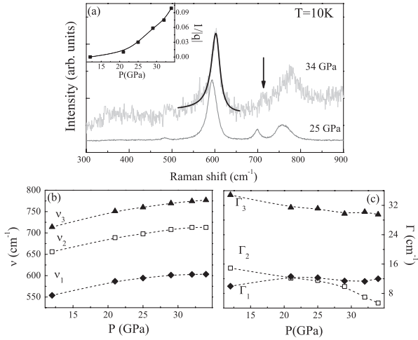
FIG. 3. (a) Raman spectra collected at 10 K at two selected pressures. Inset: Pressure dependence of the inverse of the asymmetry Fano parameter q . (b) Pressure dependence of phonon peak frequencies. (c) Pressure dependence of peak widths.
