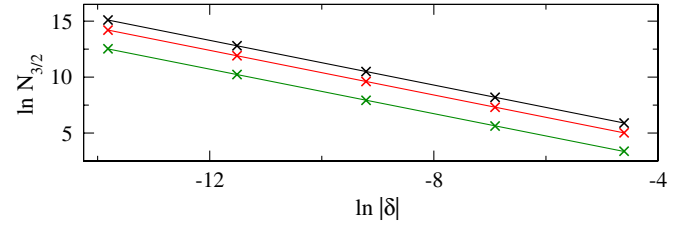
FIG. 2 (color online). Study of the crossover between the “small system limit” and the thermodynamic limit illustrated in Fig. 1. As the system size is increased in Fig. 1(a), the slope of the curves changes smoothly from 2 (corresponding to \ln \mathcal{F} \sim -N^2 ) to 1 (corresponding to \ln \mathcal{F} \sim -N ). The crossover region between the two limits is centered around N = N_{3/2} where the slope equals 3/2. To find it, we have calculated numerically \mathcal{F}(g, \delta) vs N —as in Fig. 1(a)—for various \delta ’s and found that N_{3/2}|\delta| \sim 1 . This is illustrated in this figure where data sets from top to bottom correspond to results obtained for g = 1, 1 + \delta and 1 + 5\delta , respectively [similarly as in Fig. 1(a)]. The power-law fits (straight lines) to numerical data (crosses) give N_{3/2} = a|\delta|^{-b} , where b = 0.995 \pm 0.003 for all three fits, while the prefactor a changes between the fits from 3.6 to 0.3. Similar analysis can be done on curves shown in Fig. 1(b) providing the same result. Thus, we conclude that the crossover condition reads N|\delta| \sim 1 near the Ising critical point.
