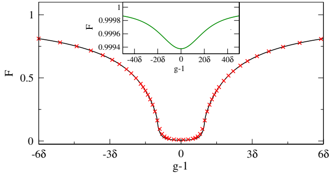
FIG. 3 (color online). Fidelity \mathcal{F}(g, \delta) of the Ising chain near the critical point: thermodynamic limit (main plot) vs “small system limit” (inset). Main plot: black curve is our analytic approximation (6), while red crosses come from numerics. Both were obtained for N = 2 \times 10^5 and \delta = 10^{-4} ( N|\delta| \gg 1 ). Inset: numerical result for N = 10^3 and \delta = 10^{-4} ( N|\delta| \ll 1 ). In the “small system limit” fidelity stays close to unity at any distance from the critical point, while in the thermodynamic limit it can interpolate between zero and unity.
