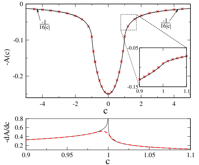
FIG. 4 (color online). Upper plot: scaling function A(c) of the Ising chain. The black line provides the analytic result (7), while the red crosses show numerics (i.e., \ln \mathcal{F}/N|\delta| ). The inset highlights singularity at c = 1 . Lower plot: logarithmic divergence of dA/dc|_{c=1} discussed in the text. The solid black line is the derivative of (7), while the red dashed line is a numerical result: the difference between the two near the pinch point at c = 1 is due to the finite system size N [19]. It disappears for N \rightarrow \infty . In both plots numerics is done for N = 10^5 and \delta = \pi 10^{-3} .
