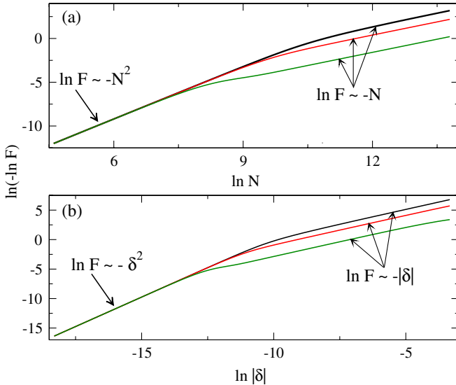
FIG. 1 (color online). Fidelity of the Ising chain near the critical point as a function of (a) the system size N at fixed \delta = 10^{-4} and (b) parameter difference \delta at the fixed system size N = 10^5 . On both panels the curves from top to bottom correspond to \mathcal{F}(1, \delta) , \mathcal{F}(1 + \delta, \delta) and \mathcal{F}(1 + 5\delta, \delta) .
