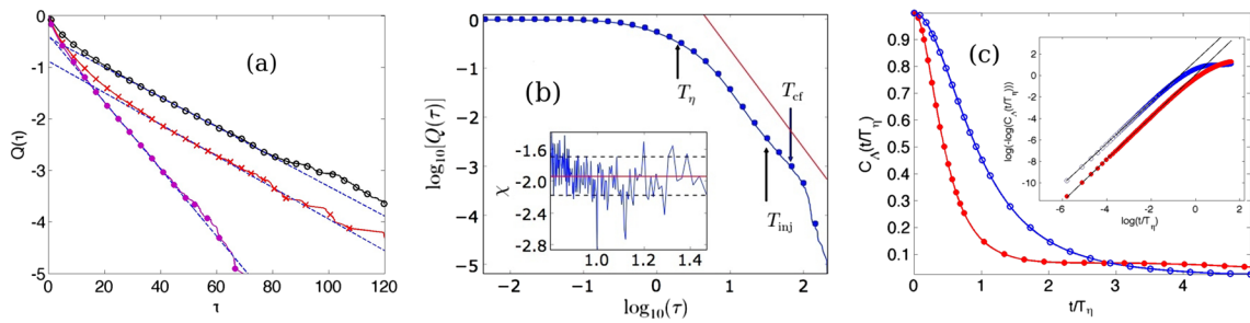
FIG. 2 (color online). (a) Representative semilog plots (base 10) of the cumulative persistence-time PDFs Q_E^+ (red crosses), Q_E^- (black open circles), and Q_L^- (magenta full circles); the subscripts E and L signify Eulerian and Lagrangian frames, respectively; and the superscripts + or - distinguish PDFs from vortical points from those from extensional ones. The dashed lines indicate exponential fits to these cumulative PDFs. These plots use data from our run R4. (b) A representative log-log plot (base 10) of the cumulative PDF Q_L^+(\tau) ( \bullet ) versus \tau for our run R4; the full red line, with a slope equal to -2 , is drawn for reference. The vertical arrows indicate the time scales (from left to right) T_\eta , T_{\text{inj}} , and T_{\text{cf}} , respectively. The inset shows the local slope \chi = d\log_{10}Q_L^+(\tau)/d\log_{10}(\tau) versus \tau ; the horizontal line is drawn at the mean \langle \chi \rangle \approx -1.93 and the black dashed lines, drawn at \langle \chi \rangle \pm \sigma_\chi , where \sigma_\chi \approx 0.2 is the standard deviation of \chi . (c) Plots of the autocorrelation function of the Okubo-Weiss parameter C_\Lambda(t/T_\eta) (see text) versus t/T_\eta in Eulerian (blue open circles) and Lagrangian (red full circles) frames for our run R1. In the inset we compare the data points for these plots with their fits (full lines) to the form G \exp[-(t/T_\Lambda)^2] .
