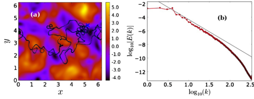
FIG. 1 (color online). (a) A pseudocolor plot of the stream function \psi , at a representative time in the statistically steady state, with a representative Lagrangian-particle track (blue squares) superimposed on it from our run R2. The symbol \circ indicates the beginning of the trajectory and the \times sign marks its end. For an animated version, see the movie file at [16]. (b) log-log (base 10) plot of the energy spectrum for our run R4 (line with dots); the black line with a slope -3.6 is shown for reference.
