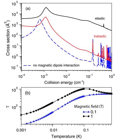
FIG. 4 (color online). (a) Cross sections for elastic scattering (black line) and inelastic relaxation (red line) in NH + N collisions calculated as functions of collision energy at an average magnetic field of 0.1 \text{ T} experienced by trapped species at a temperature of 600 \text{ mK} in the 4 \text{ T} deep trap. Also shown is the cross section calculated with the magnetic dipole interaction omitted (dashed line). (b) Thermally averaged ratios of the rate constants for elastic scattering and inelastic relaxation as functions of temperature.
