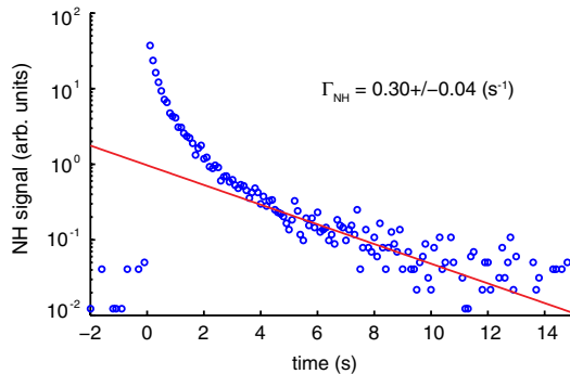
FIG. 1 (color online). NH trap decay taken at a trap depth of 3.9 T and cell temperature 570 mK. The solid line is a fit to the form n_{\text{NH}} = a \exp[-\Gamma_{\text{NH}}t] . The fit to the exponential decay was performed over the range of 5.5 to 10 s.
