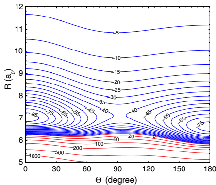
FIG. 3 (color online). Contour plot of the ab initio interaction PES for the fully spin-polarized S = 5/2 state of N + NH calculated in this work. The NH bond distance is fixed at its equilibrium value r = 1.958 a_0 . Energies are in units of \text{cm}^{-1} .
