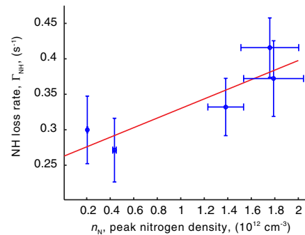
FIG. 2 (color online). NH loss rate vs cotrapped N density. The (red) line is a fit to the data to Eq. (1). The vertical error bars represent 1 standard deviation intervals from the fit for \Gamma_{\text{NH}} as shown in Fig. 1. The horizontal error bars represent the change in N density over the interrogation time of 5.5 to 10 s. The calibration of the peak N density (horizontal axis scale) contains an overall uncertainty of 30%.
