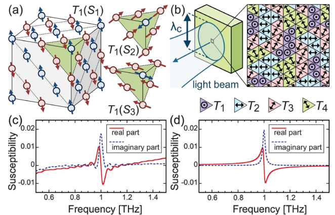
FIG. 2 (color). (a) Schematics of spin alignment in three S domains belonging to the T_1 domain, and (b) random distribution of four orientations of T domains within the coherent length \lambda_c of the light beam. (c) Experimental and (d) calculated magnetic susceptibility of NiO; \Gamma = 70 GHz and \varepsilon_r = 12.25 are assumed.
