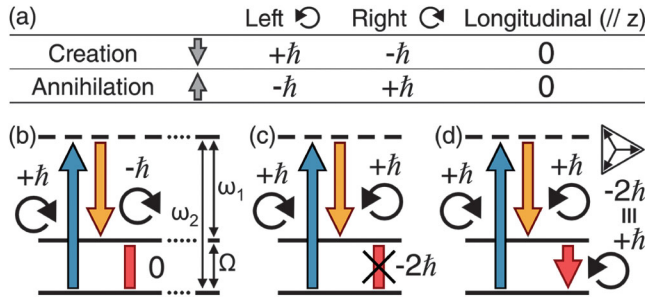
FIG. 1 (color). (a) Changes of J_z^{\text{EM}} by creation or annihilation of photons propagating along the z axis. The lower panels show schematics of the changes of the angular momentum in collinear scattering processes of photons to a mode with (b) the same helicity and (c) the opposite, and (d) a collinear DFG process allowed along a threefold axis involving two photons with opposite helicity.
