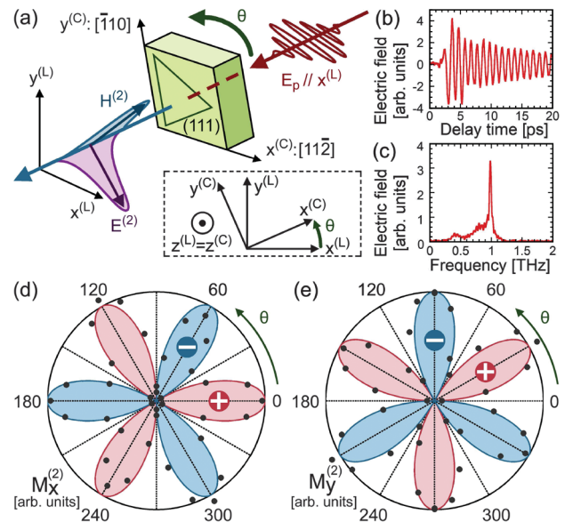
FIG. 3 (color). (a) Schematics of the experimental setup. The inset shows the relation between crystal and laboratory coordinates. (b) Temporal waveform of the radiation from NiO and (c) its Fourier transformed spectrum. Polar plots of the transverse components (d) M_x^{(2)} and (e) M_y^{(2)} of the induced magnetization as functions of the crystal rotation angle \theta . The dots are experimental data of their amplitude, and the solid curves are calculated by Eq. (11).
