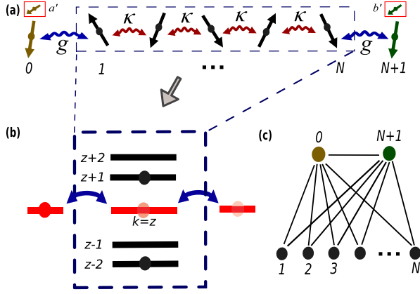
FIG. 1 (color online). (a) Distant spin qubits coupled by an unpolarized spin-chain quantum channel with g , the coupling between qubits (yellow, green) and the spin chain, and \kappa , the coupling between intrachain elements. Boxed spins, labeled a' and b' , represent additional spin qubits that can correspond to the memory of a quantum register or ancillary qubits associated with quantum information encoding. (b) The spin chain can be reexpressed in terms of free fermions via the Jordan-Wigner transformation, wherein the hopping strength is characterized by \kappa . By ensuring that the end spins are resonant with a single fermionic mode ( k = z ), unpolarized spin-chain state transfer becomes analogous to fermionic tunneling. Maintaining g \ll \kappa/\sqrt{N} ensures that off-resonant coupling to other fermionic modes can be neglected and enables state transfer independent of the intermediate spin-chain state. (c) Graphlike state generated by FFST between the qubits and the intermediate spin chain [20]. Each line represents a controlled-phase gate.
