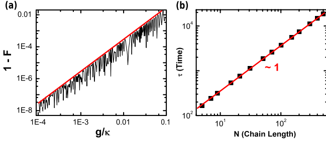
FIG. 2 (color online). (a) Numerical simulation of the infidelity of QST for N = 7 as a function of g/\kappa depicting fluctuations in the infidelity. The upper bound of the numerical infidelity is represented by the bold line. (b) For a chosen tolerable infidelity \epsilon_0 = 10^{-3} , the minimum time \tau (in units of 1/\kappa ) required for state transfer scales linearly with chain length.
