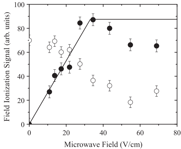
FIG. 4. Microwave field dependence of the field ionization, or recombination, signal. The phase-averaged signal (○) decreases with the microwave field. It is present, even with no microwave field, due to excitation of bound Rydberg atoms by the low frequency wing of the ps laser. The peak-to-peak phase sensitive signal, multiplied by 10 (●) rises with the microwave field to a peak at a field of 30 V/cm and then declines. The expected field dependence based on Eq. (2) and the ps laser bandwidth (solid line).
