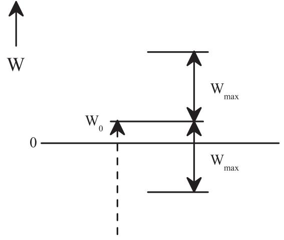
FIG. 2. If the ps laser excitation to energy W_0 occurs at \omega t_0 = \omega t_{\max} = \pi/6 , energy transfer up and down by W_{\max} occurs. If W_{\max} > W_0 , recombination can occur.
