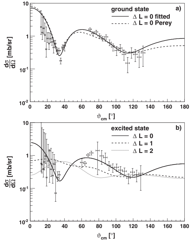
FIG. 4. Proton angular distributions for the reaction t(^{30}\text{Mg}, p)^{32}\text{Mg} populating the ground state (a) and the 1058 keV state (b). The curves in panel a) are from DWBA calculations with fitted (solid) and global (dashed) optical model parameters [34]. Panel b) includes DWBA calculations for \Delta L = 0 (solid), \Delta L = 1 (dashed) and \Delta L = 2 (dotted) transfer. The angle range around \vartheta_{\text{cm}} = 50^\circ corresponds to \vartheta_{\text{lab}} = 90^\circ which is not covered by the T-REX detector.
