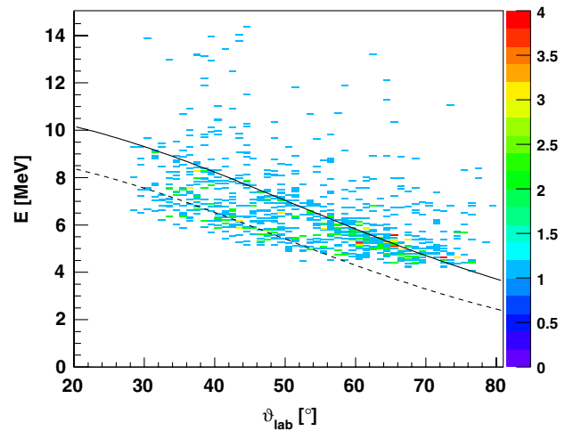
FIG. 1 (color online). Energy versus \vartheta_{\text{lab}} spectrum for ^{30}\text{Mg} on the tritium target for unambiguously identified protons. The two lines show the kinematic curves for the ground state (solid) and an excited state at 1.1 MeV (dashed).
