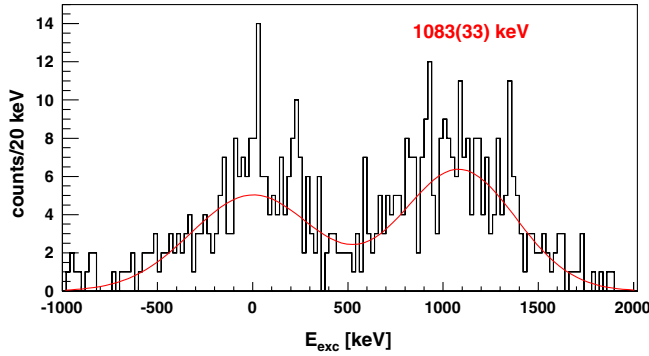
FIG. 2 (color online). Excitation energy of the ejectile ^{32}\text{Mg} reconstructed from the measured energy of protons in T-REX. The excitation energy of the observed state amounts to 1083(33) keV.
